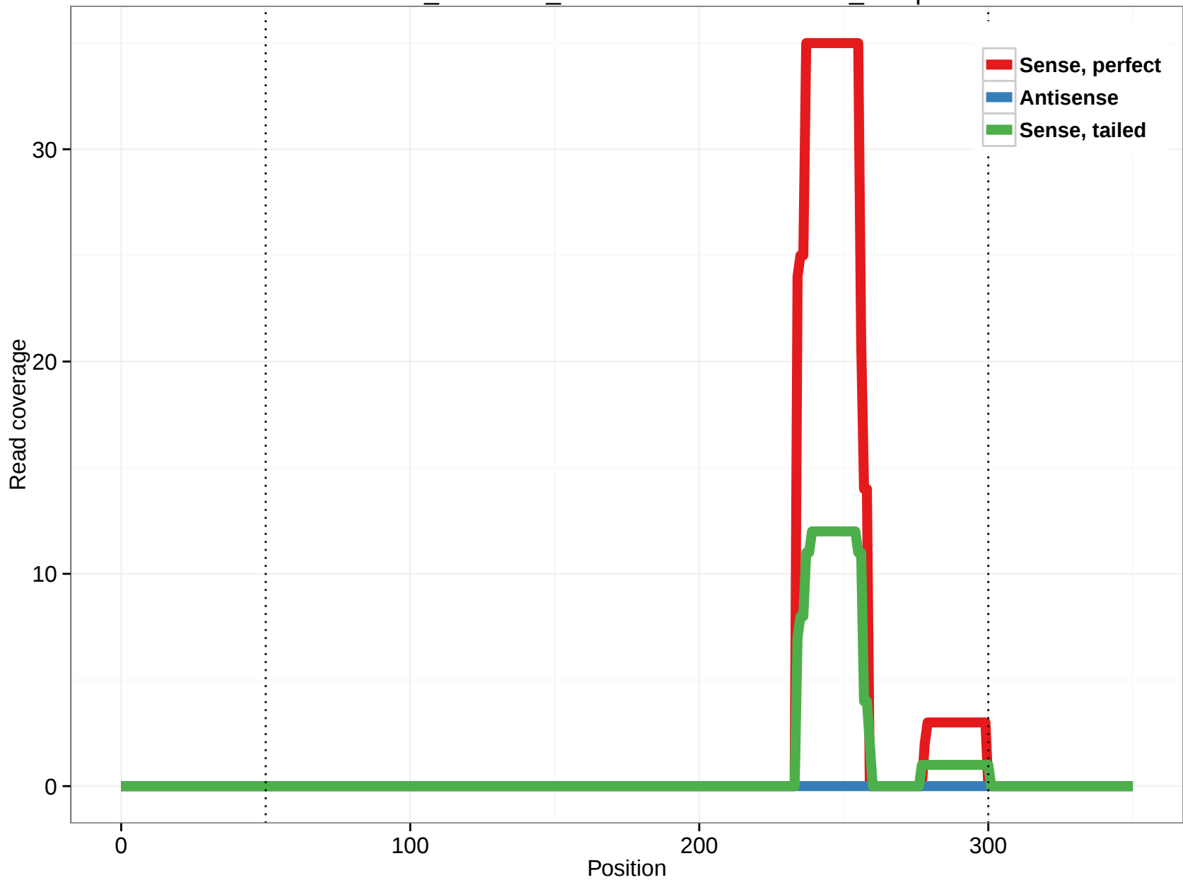
ornAna1_ensGene_ENSOANT00000019162_10.3p
