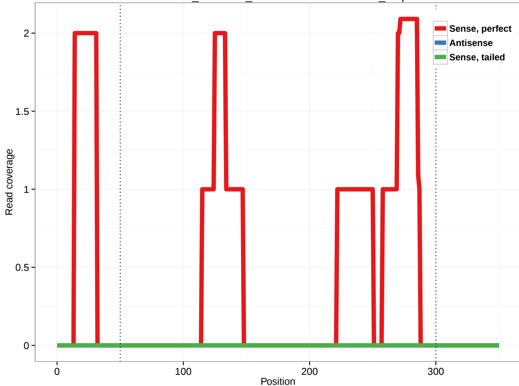
ornAna1_ensGene_ENSOANT00000019051_4.5p
