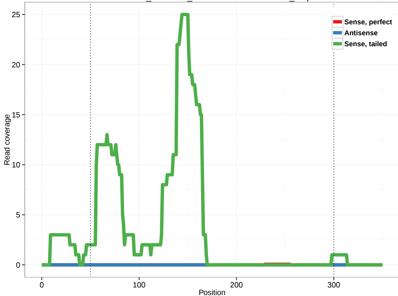
ornAna1_ensGene_ENSOANT00000018992_5.3p
