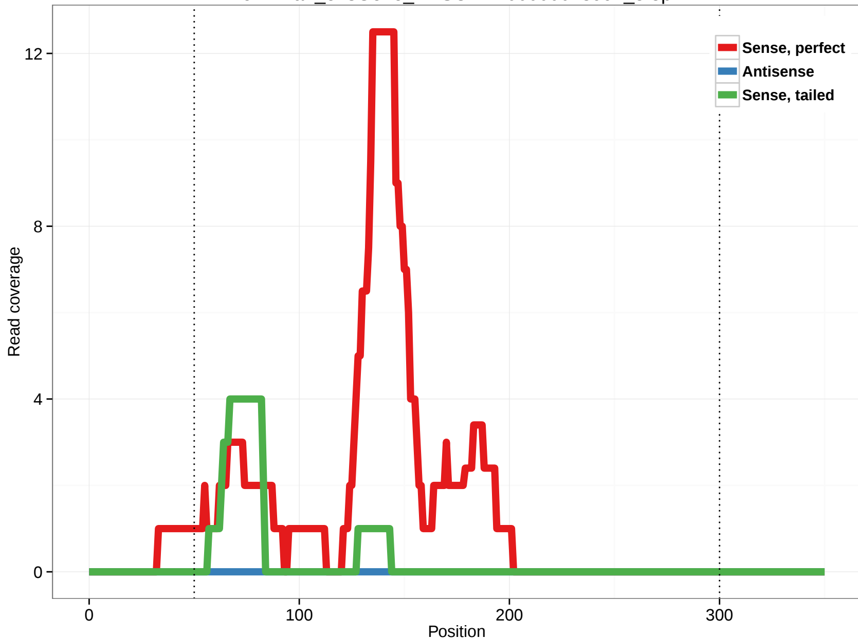
ornAna1_ensGene_ENSOANT00000018991_5.5p
