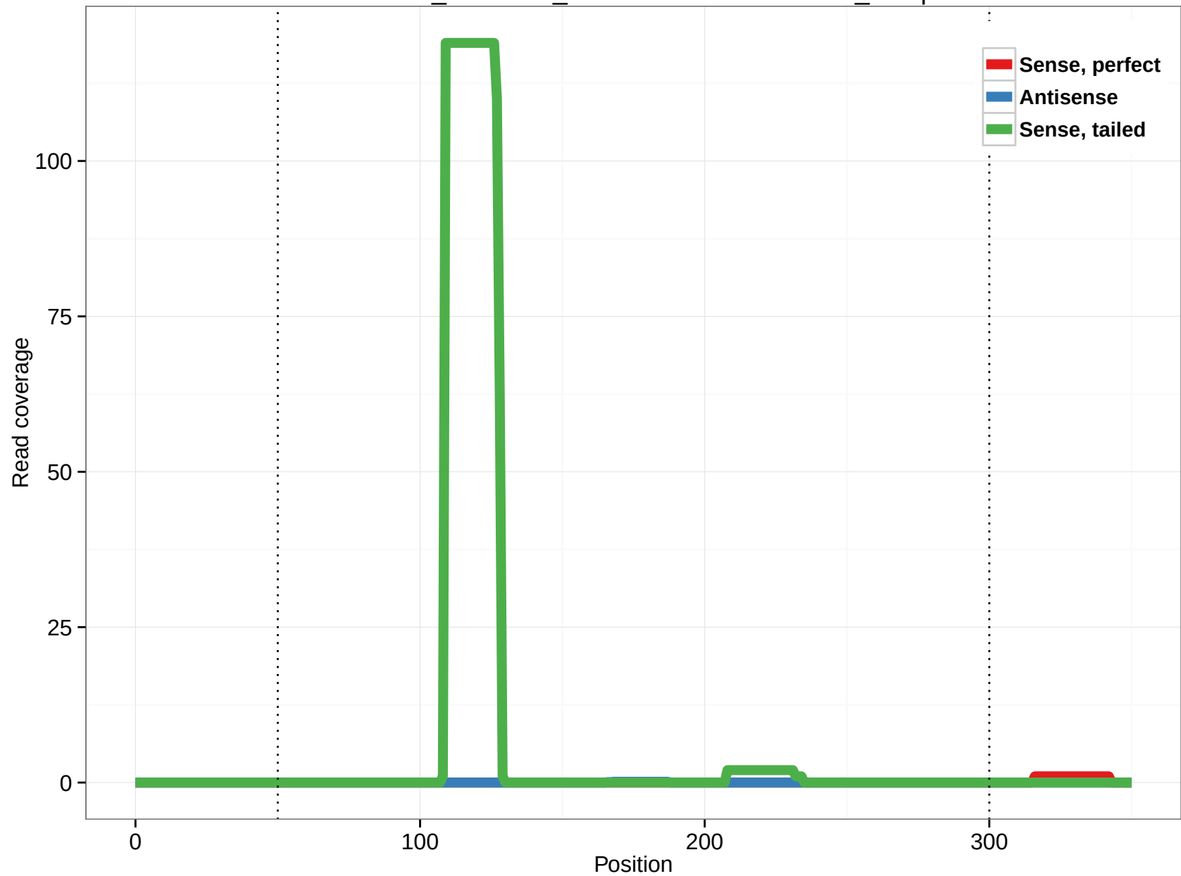
ornAna1_ensGene_ENSOANT00000018989_40.3p
