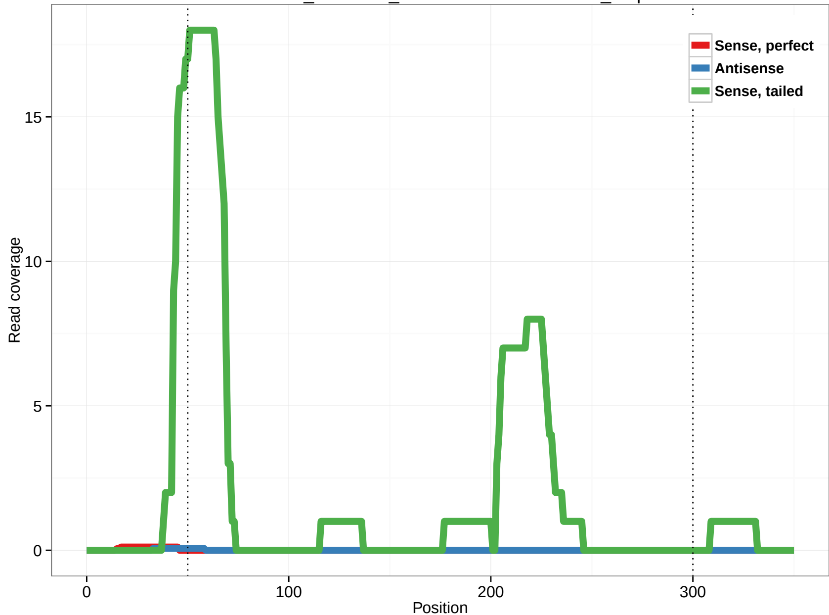
ornAna1_ensGene_ENSOANT00000018886_0.5p
