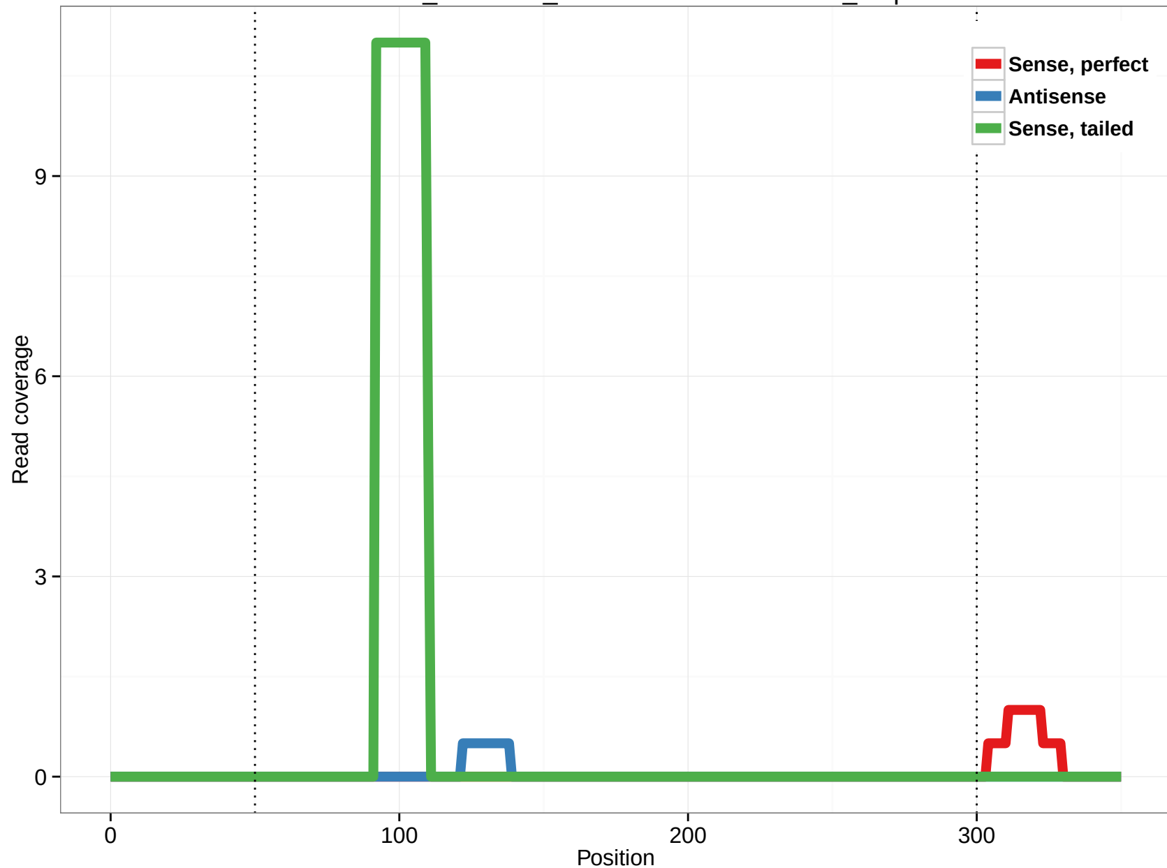
ornAna1_ensGene_ENSOANT00000018815_2.3p
