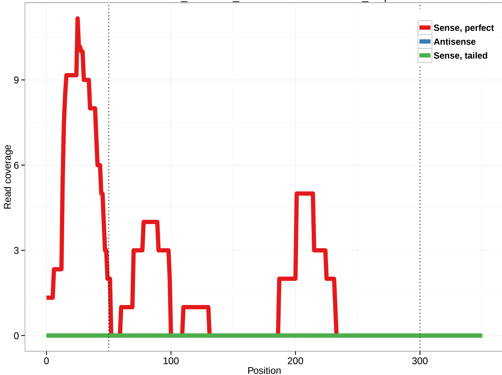
ornAna1_ensGene_ENSOANT00000018794_1.5p
