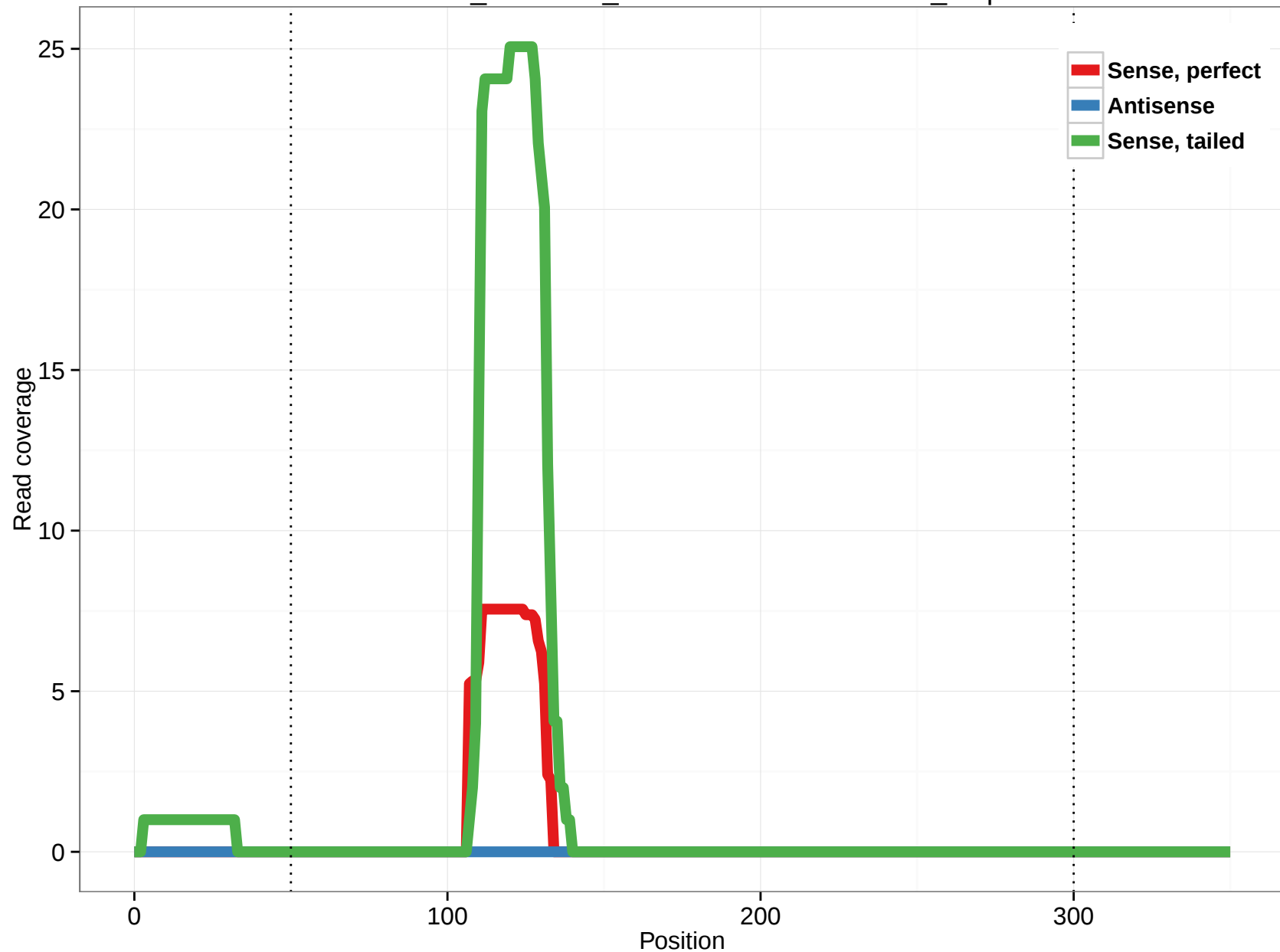
ornAna1_ensGene_ENSOANT00000018785_3.5p
