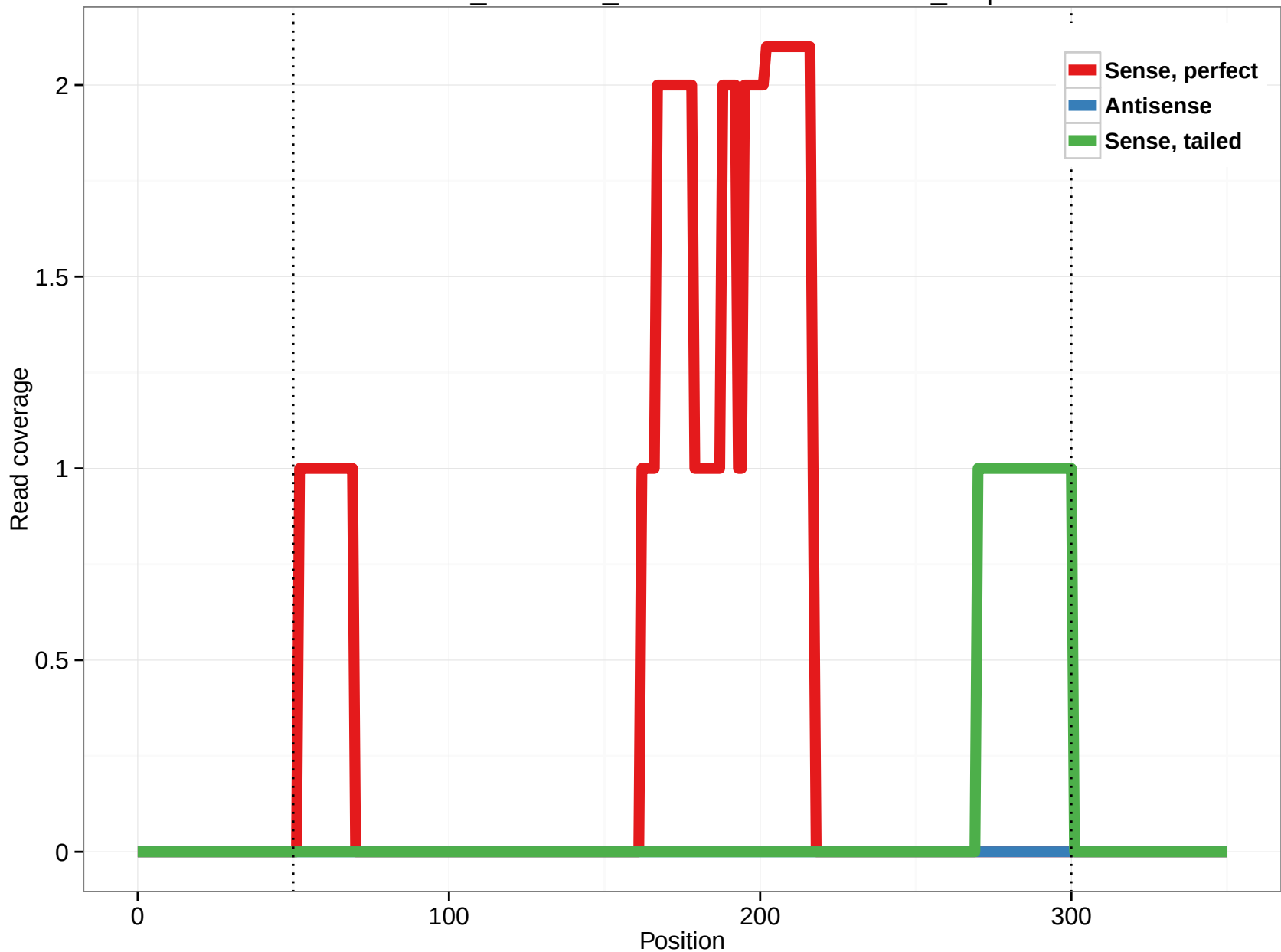
ornAna1_ensGene_ENSOANT00000018728_1.3p
