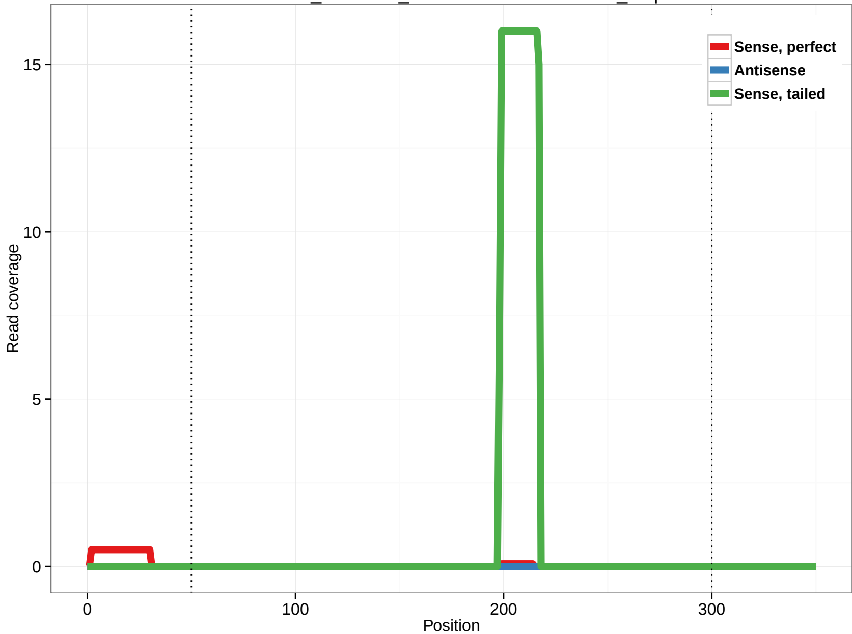
ornAna1_ensGene_ENSOANT00000018665_3.5p
