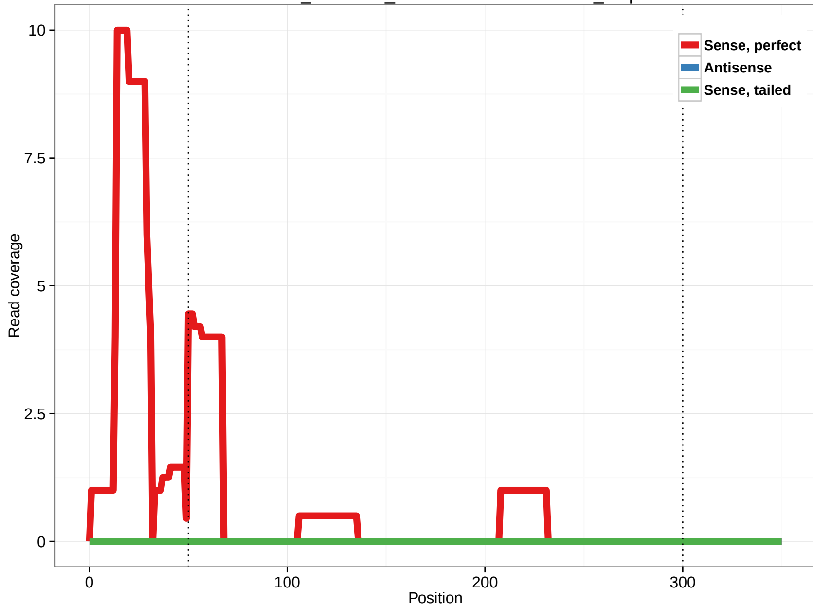
ornAna1_ensGene_ENSOANT00000018644_0.5p
