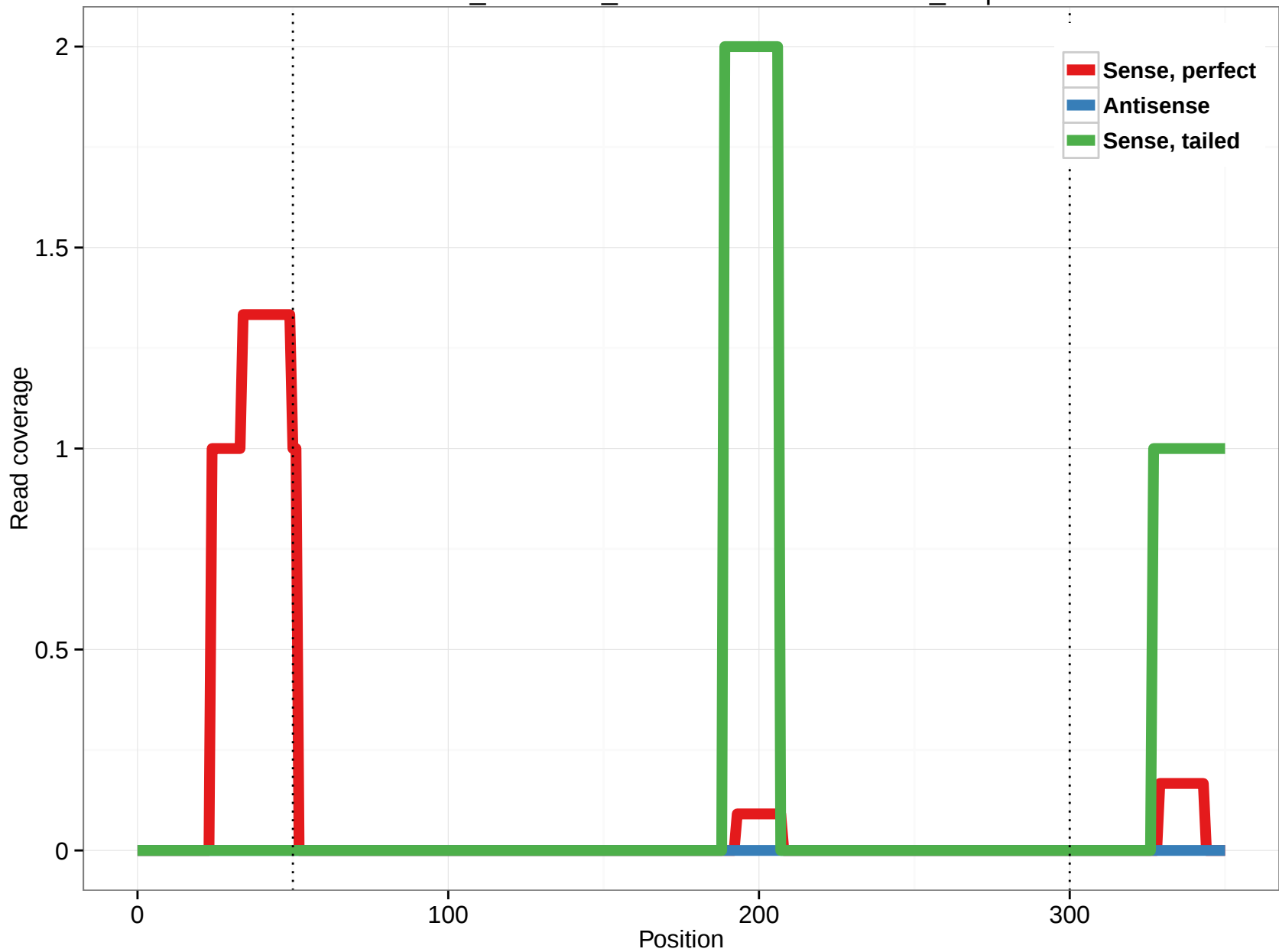
ornAna1_ensGene_ENSOANT00000018624_4.3p
