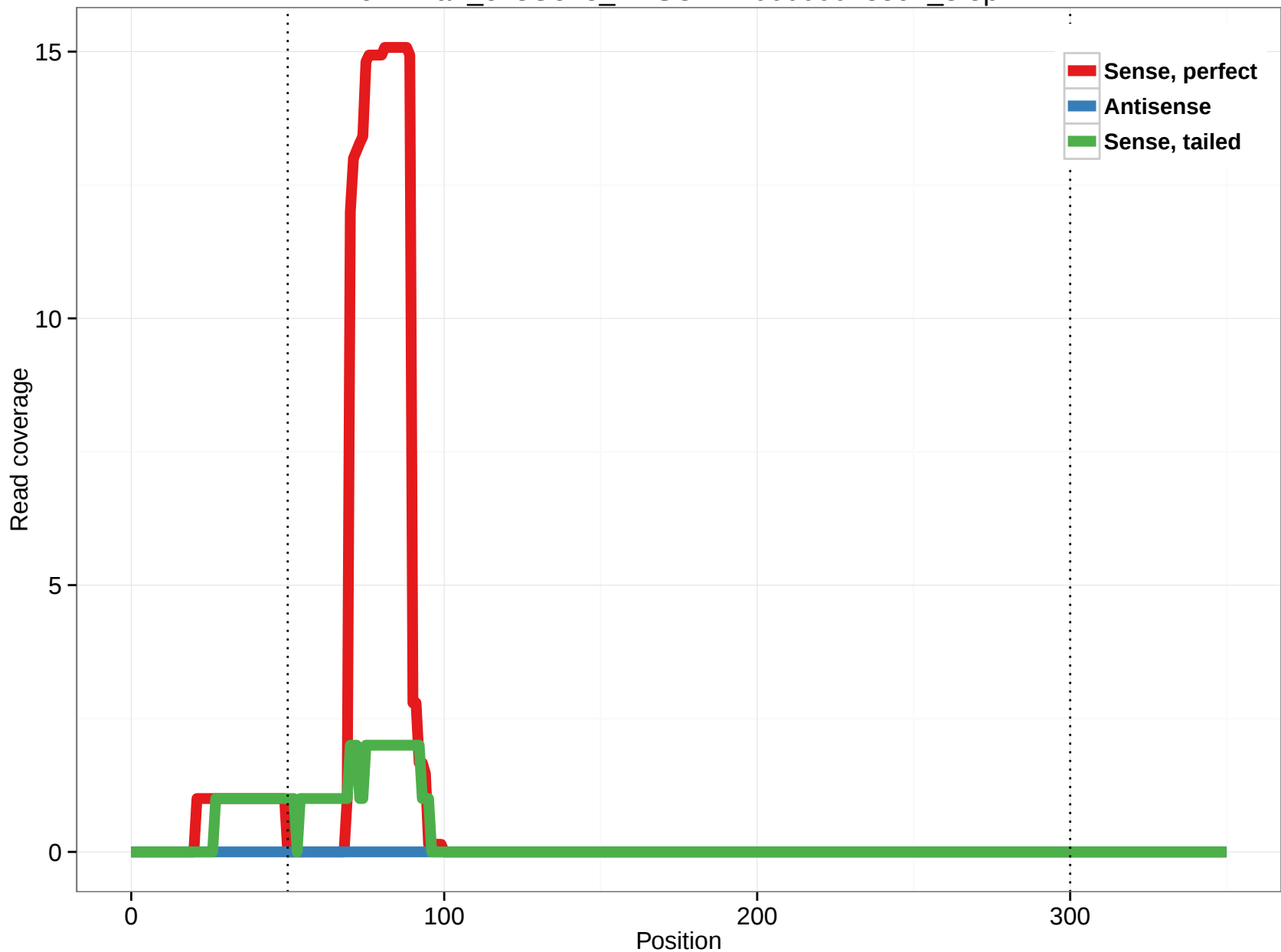
ornAna1_ensGene_ENSOANT00000018597_3.5p
