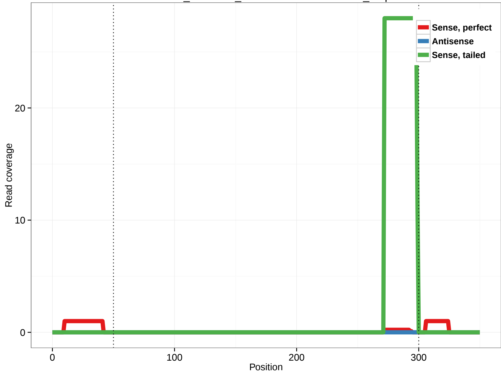
ornAna1_ensGene_ENSOANT00000018513_5.3p
