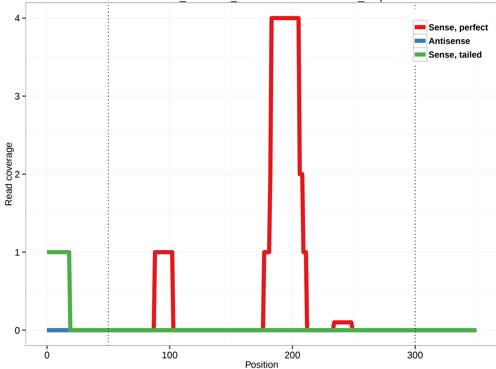
ornAna1_ensGene_ENSOANT00000018490_7.5p
