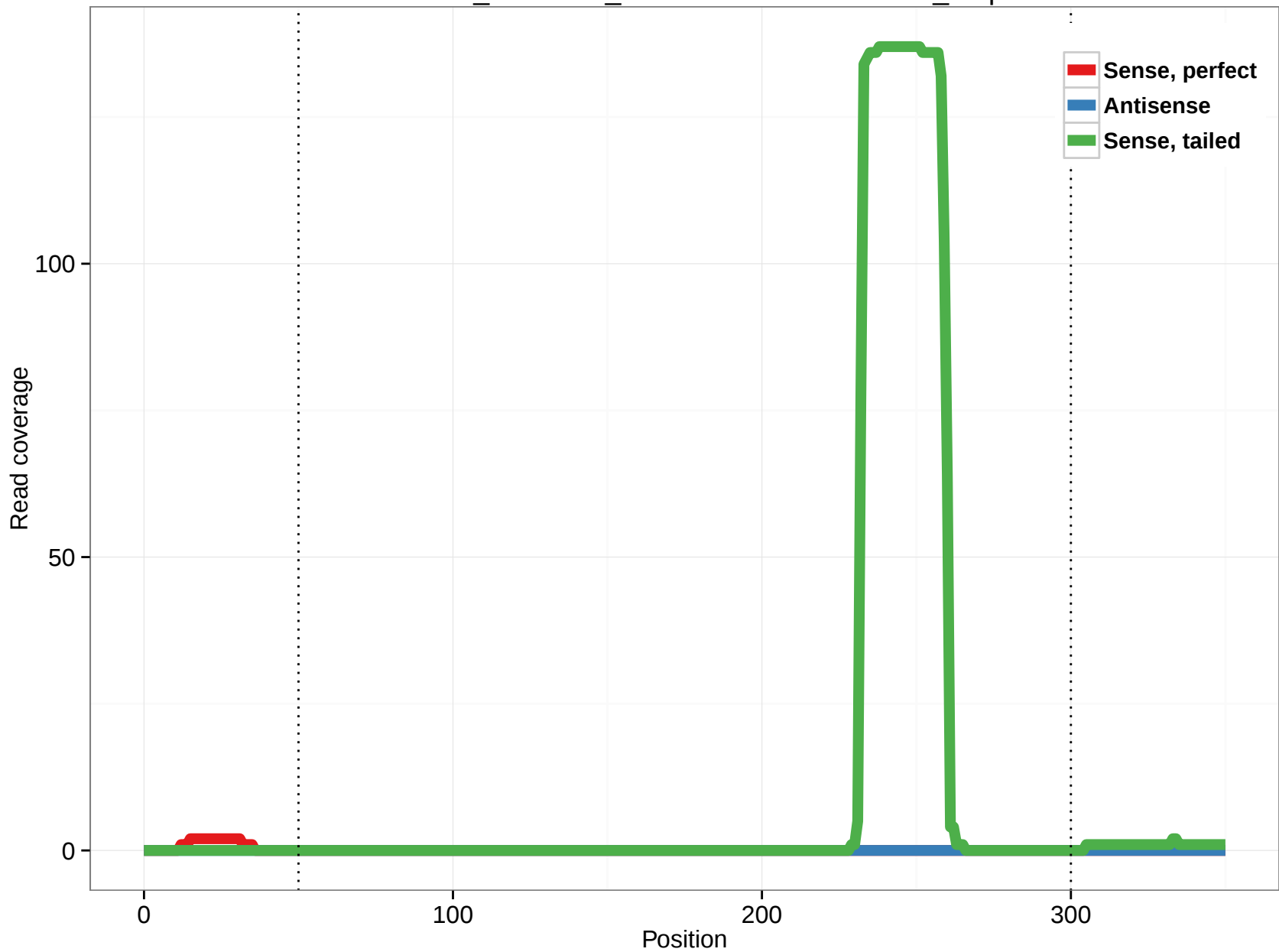
ornAna1_ensGene_ENSOANT00000018447_0.5p
