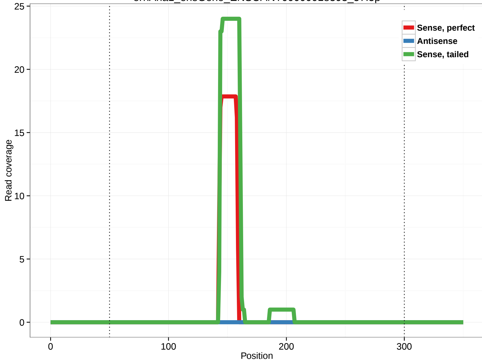
ornAna1_ensGene_ENSOANT00000018393_57.5p
