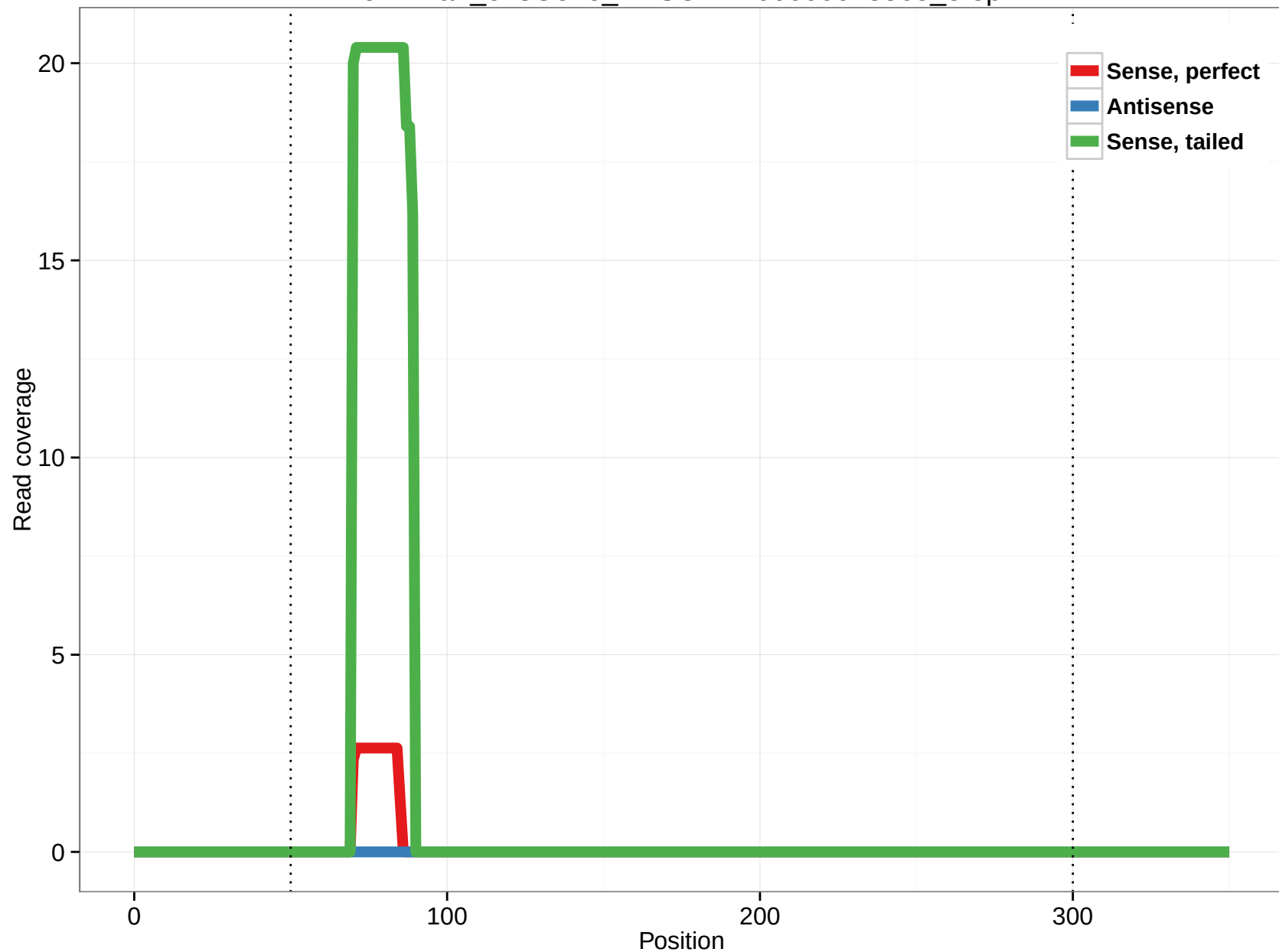
ornAna1_ensGene_ENSOANT00000018365_3.3p
