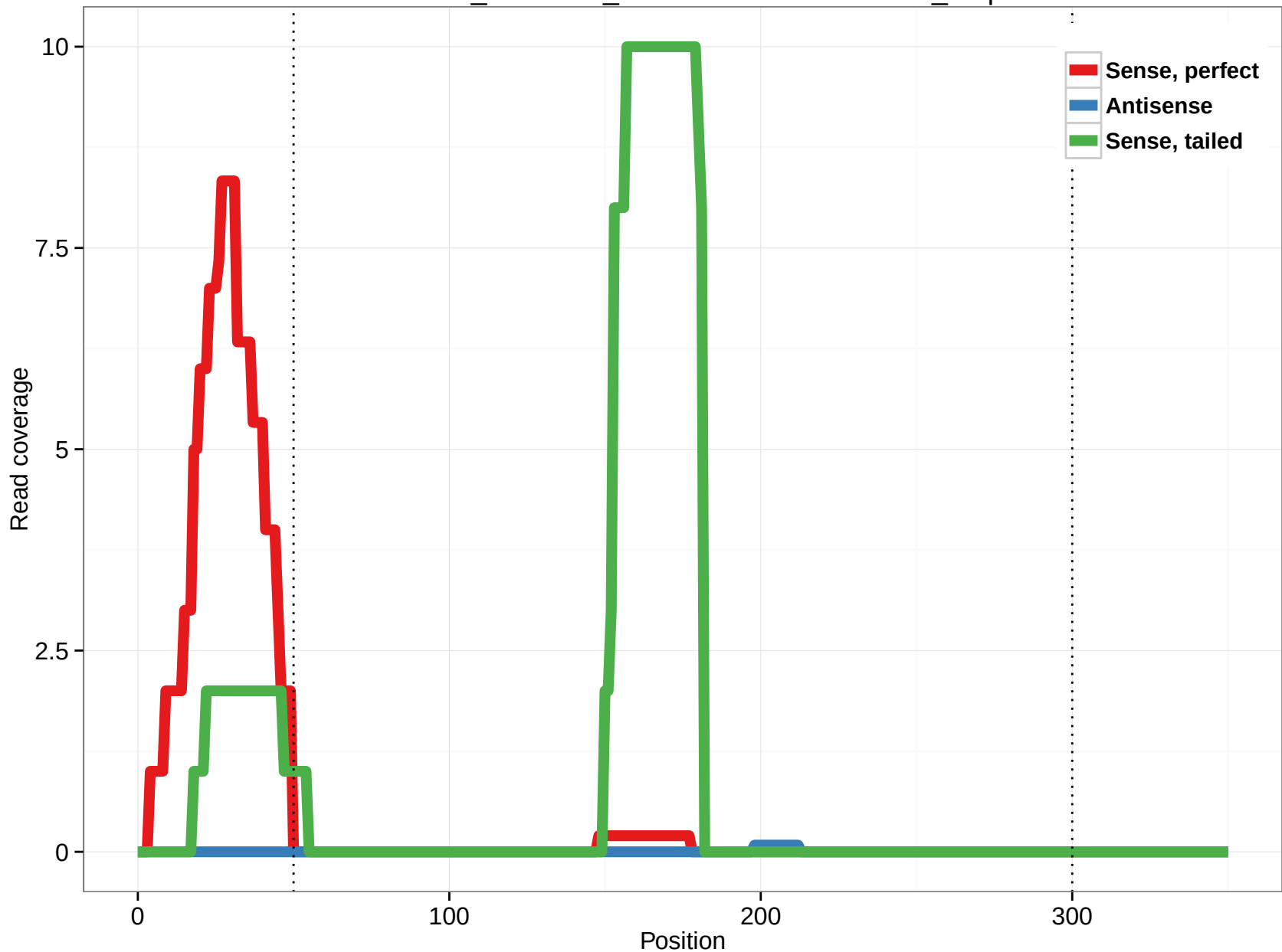
ornAna1_ensGene_ENSOANT00000018360_0.5p
