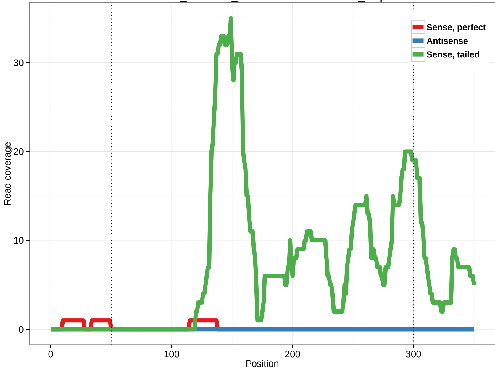
ornAna1_ensGene_ENSOANT00000018344_7.5p
