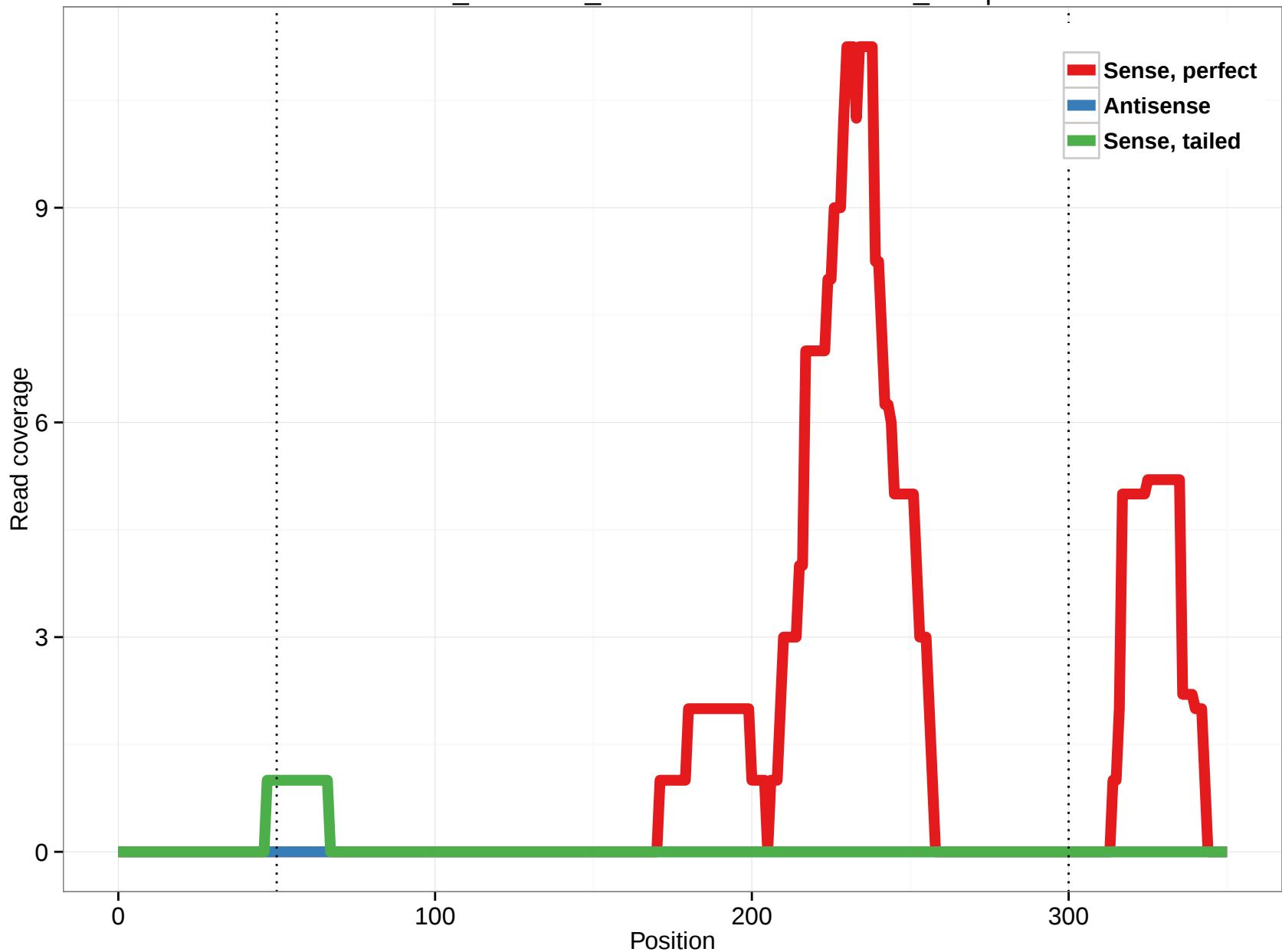
ornAna1_ensGene_ENSOANT00000018324_13.5p
