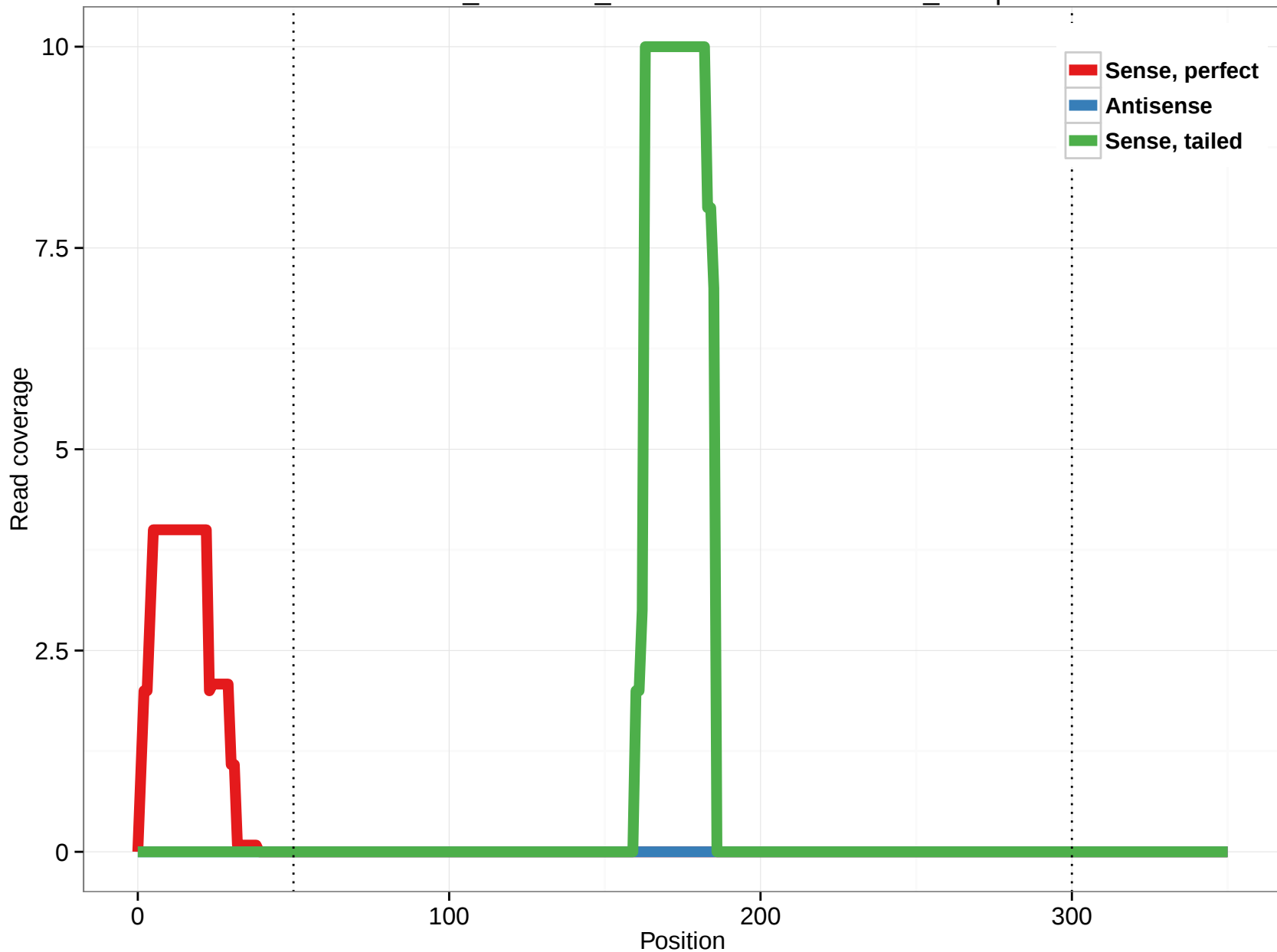
ornAna1_ensGene_ENSOANT00000018289_20.5p
