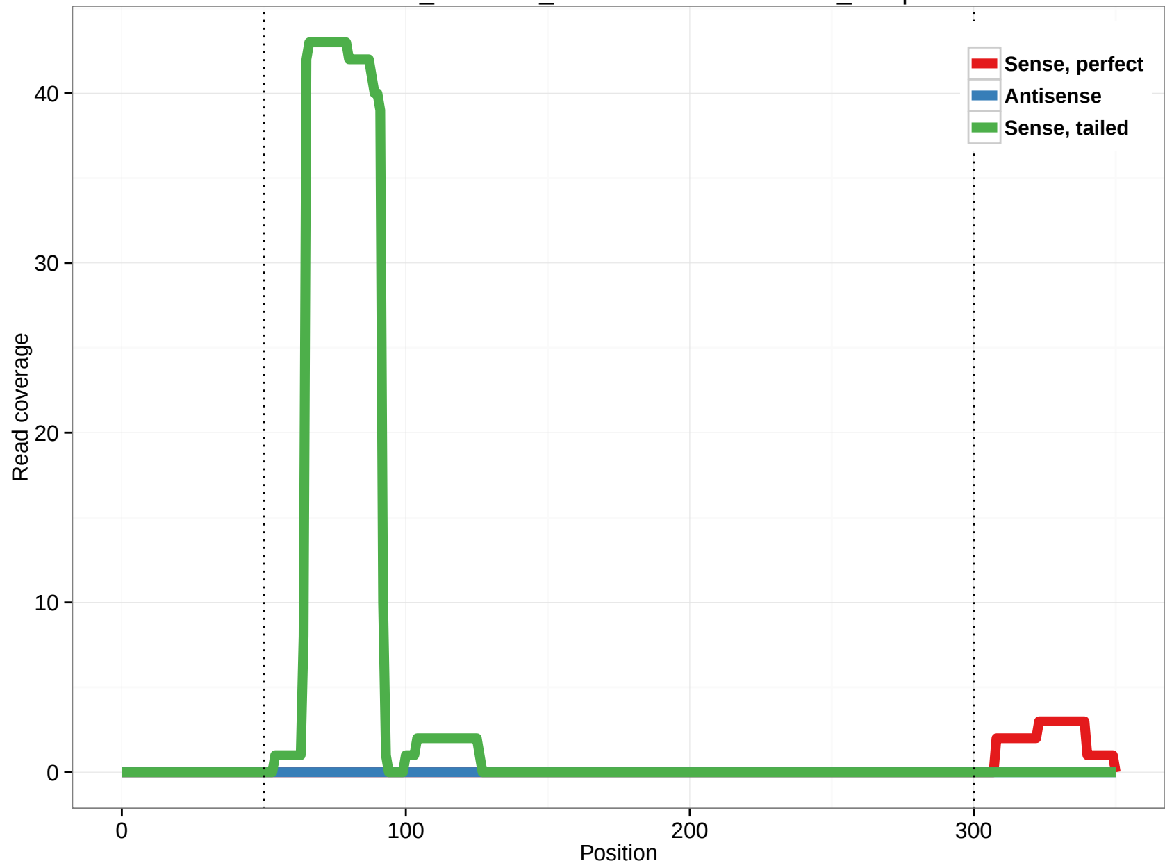
ornAna1_ensGene_ENSOANT00000018289_12.3p
