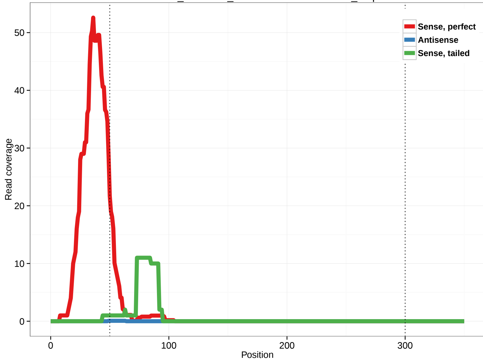
ornAna1_ensGene_ENSOANT00000018278_0.5p
