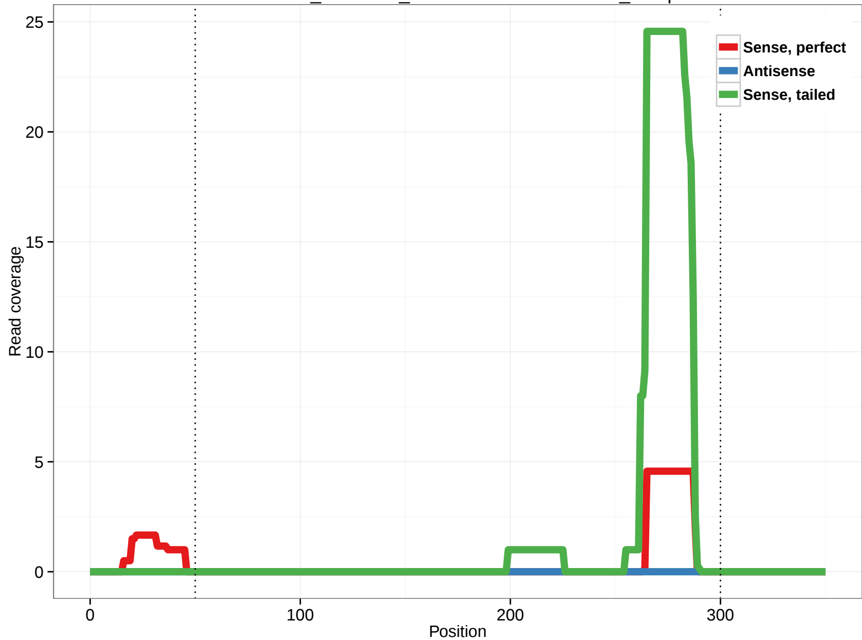
ornAna1_ensGene_ENSOANT00000018239_20.5p
