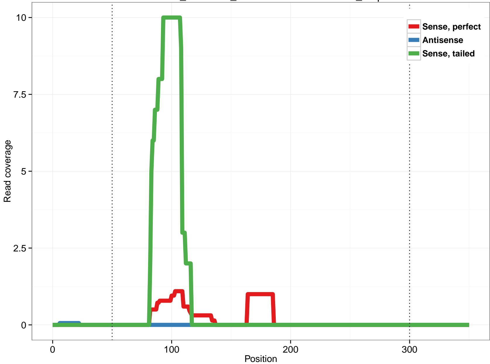
ornAna1_ensGene_ENSOANT00000018226_0.3p
