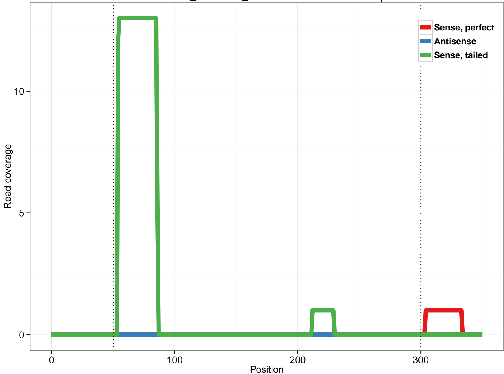
ornAna1_ensGene_ENSOANT00000018202.3p
