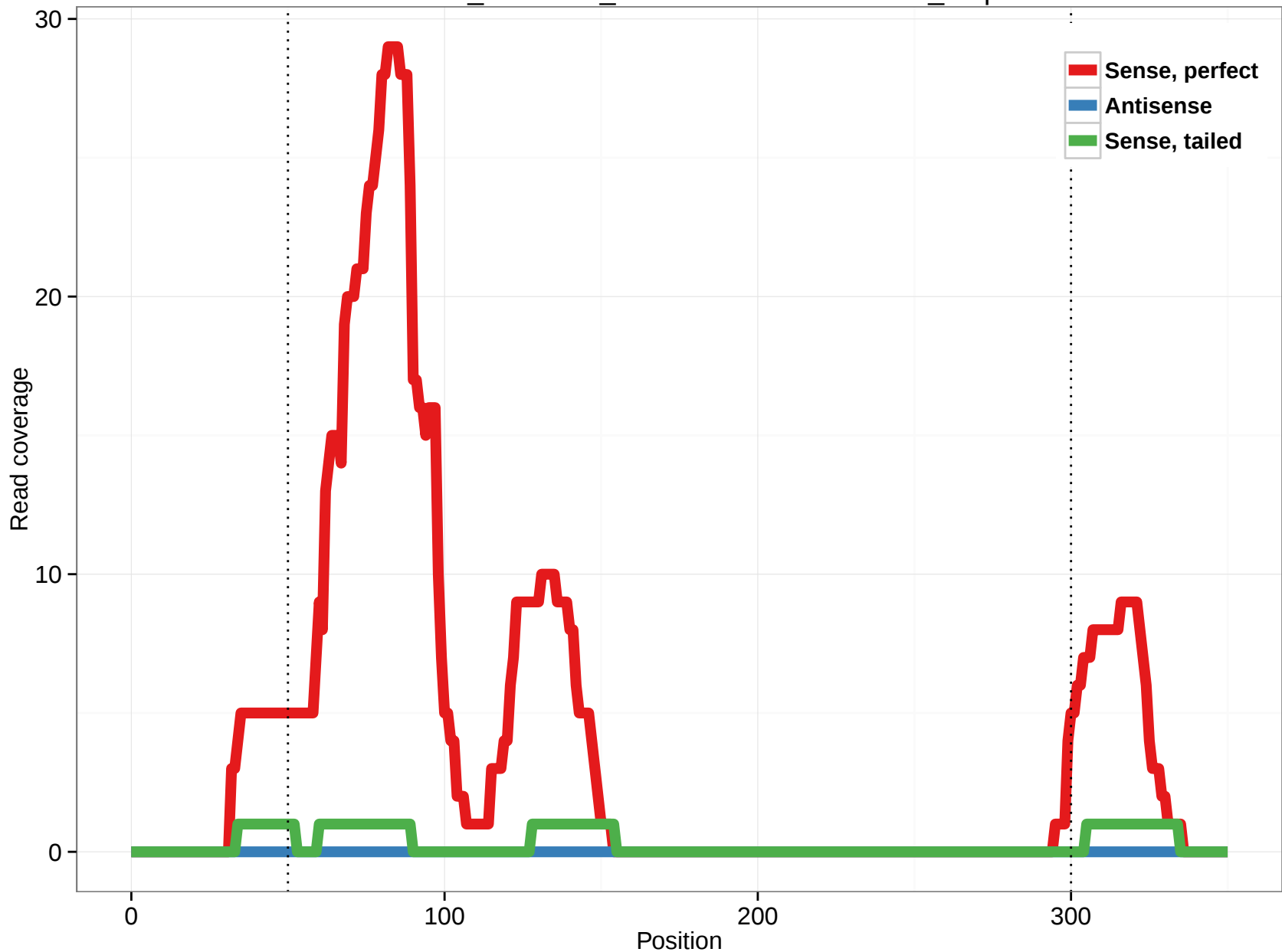
ornAna1_ensGene_ENSOANT00000018123_0.3p
