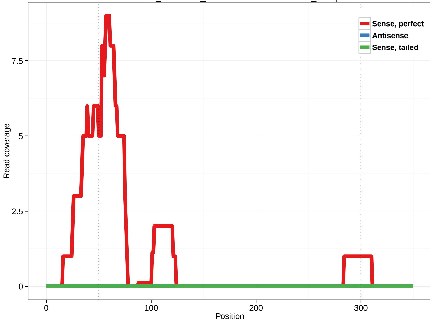
ornAna1_ensGene_ENSOANT00000018101_13.5p
