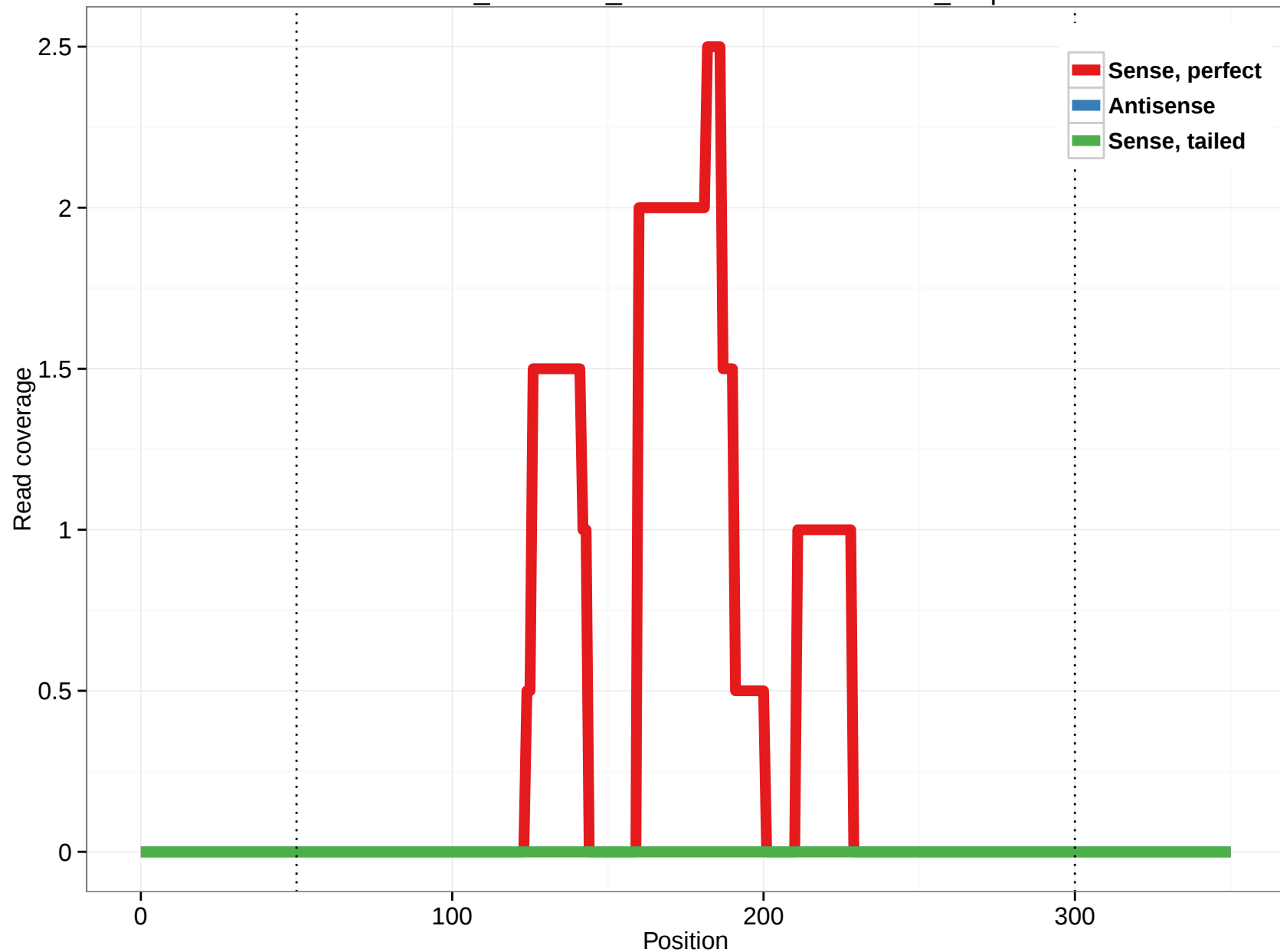
ornAna1_ensGene_ENSOANT00000018100_7.3p
