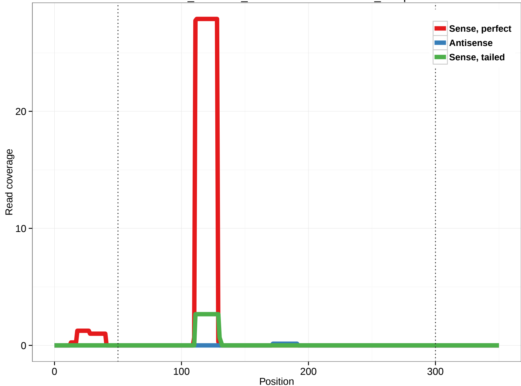
ornAna1_ensGene_ENSOANT00000018064_10.5p
