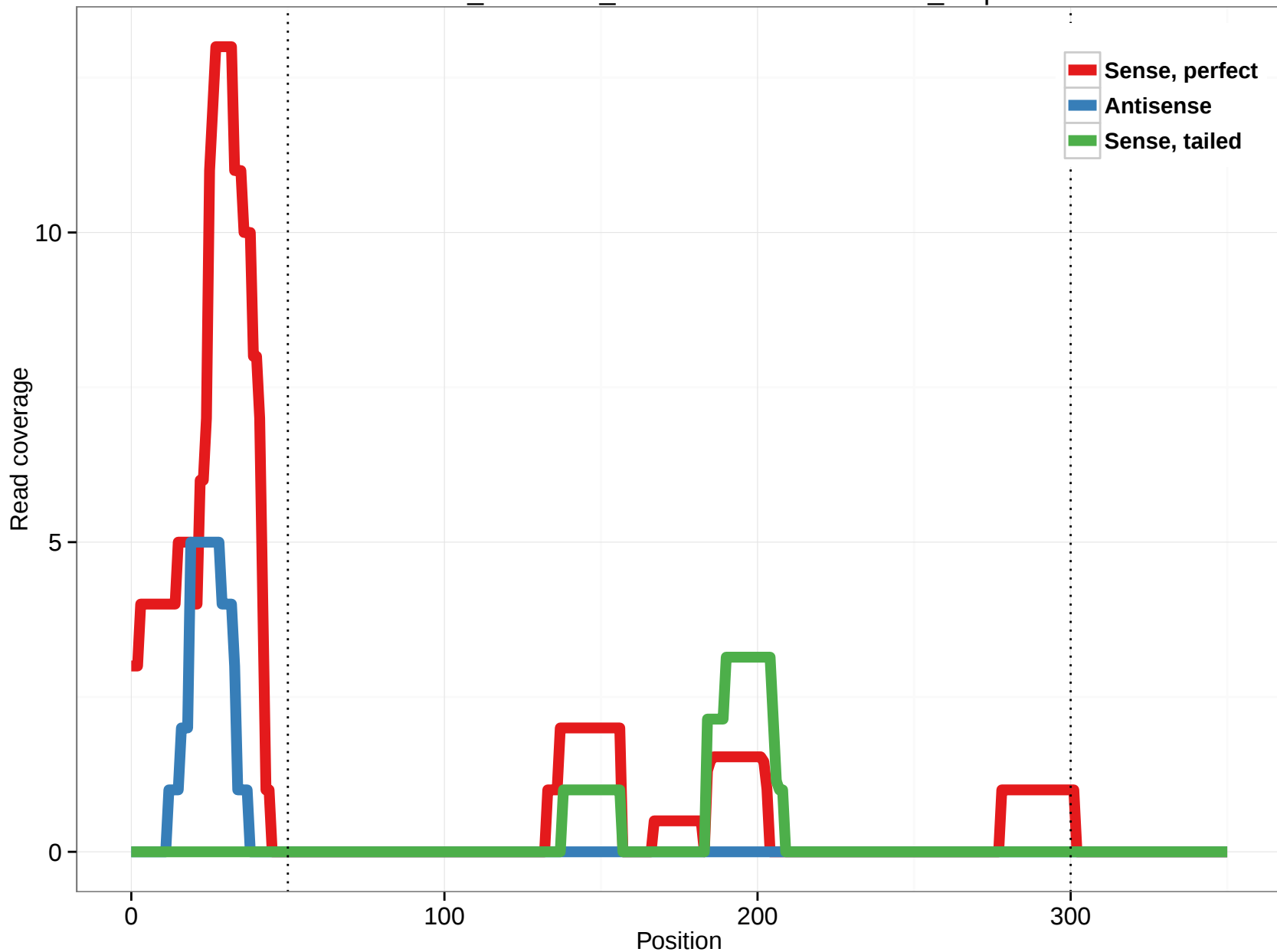
ornAna1_ensGene_ENSOANT00000018044_4.5p
