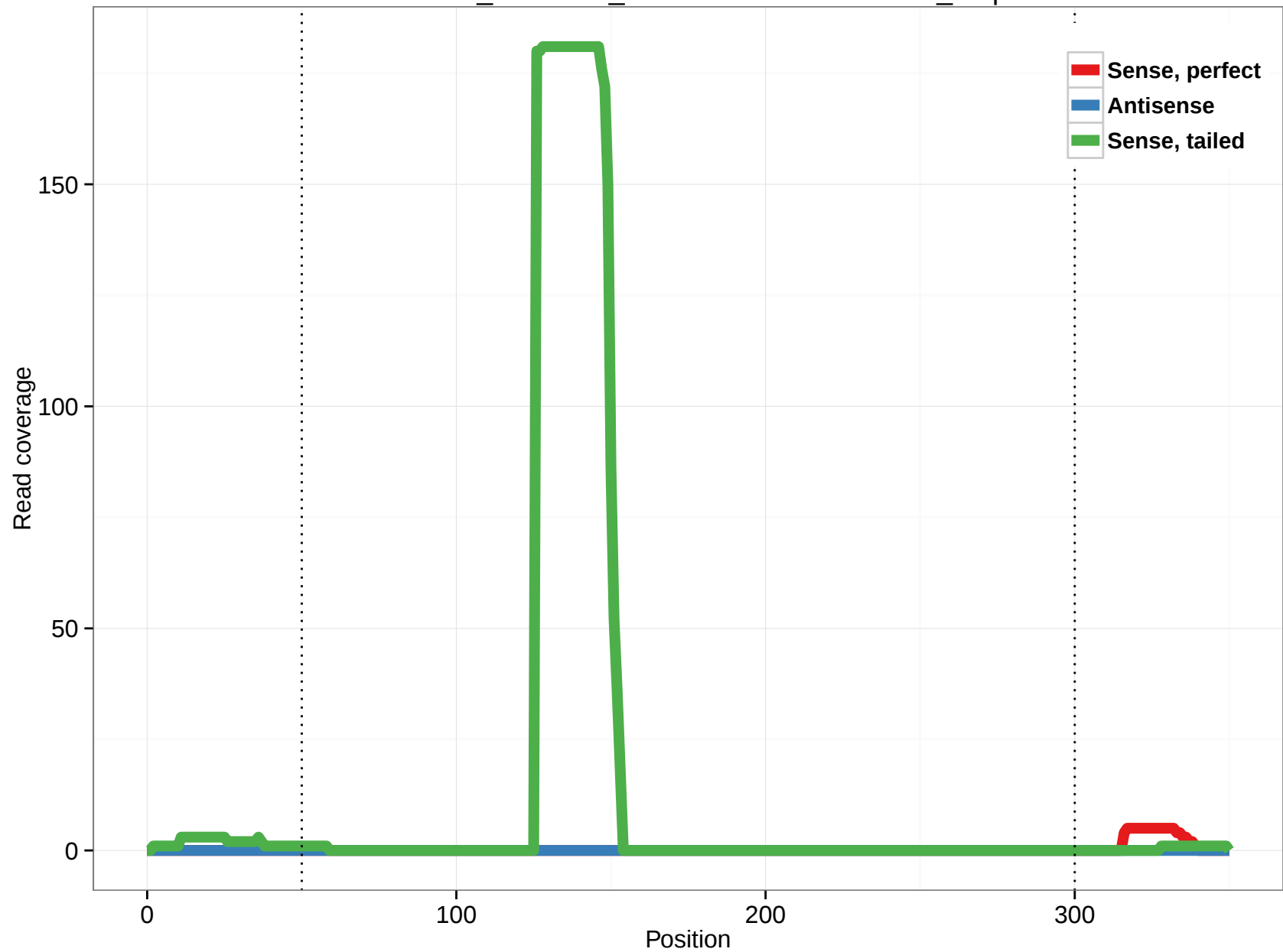
ornAna1_ensGene_ENSOANT00000018007_3.3p
