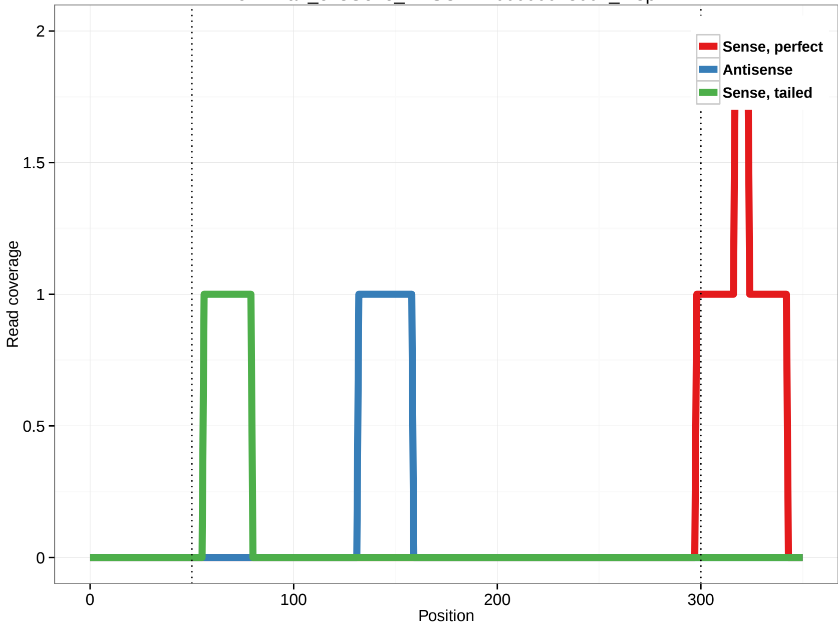
ornAna1_ensGene_ENSOANT00000018004_7.3p
