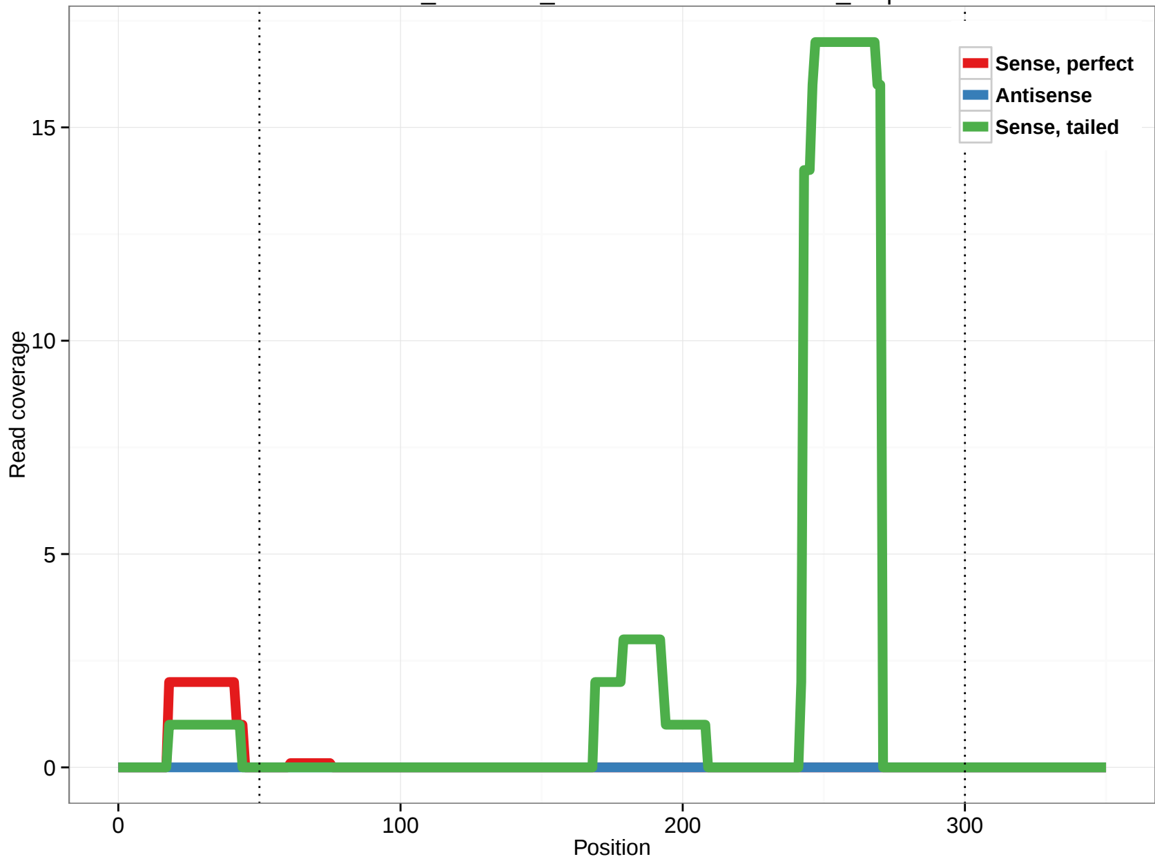
ornAna1_ensGene_ENSOANT00000017950_3.5p
