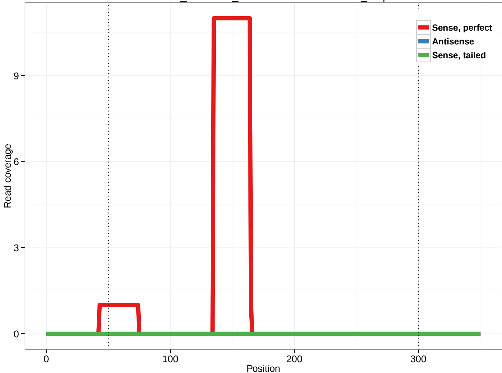
ornAna1_ensGene_ENSOANT00000017895_2.3p
