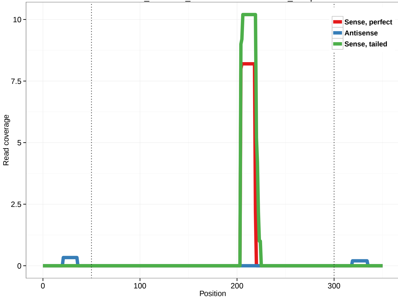
ornAna1_ensGene_ENSOANT00000017887_21.5p
