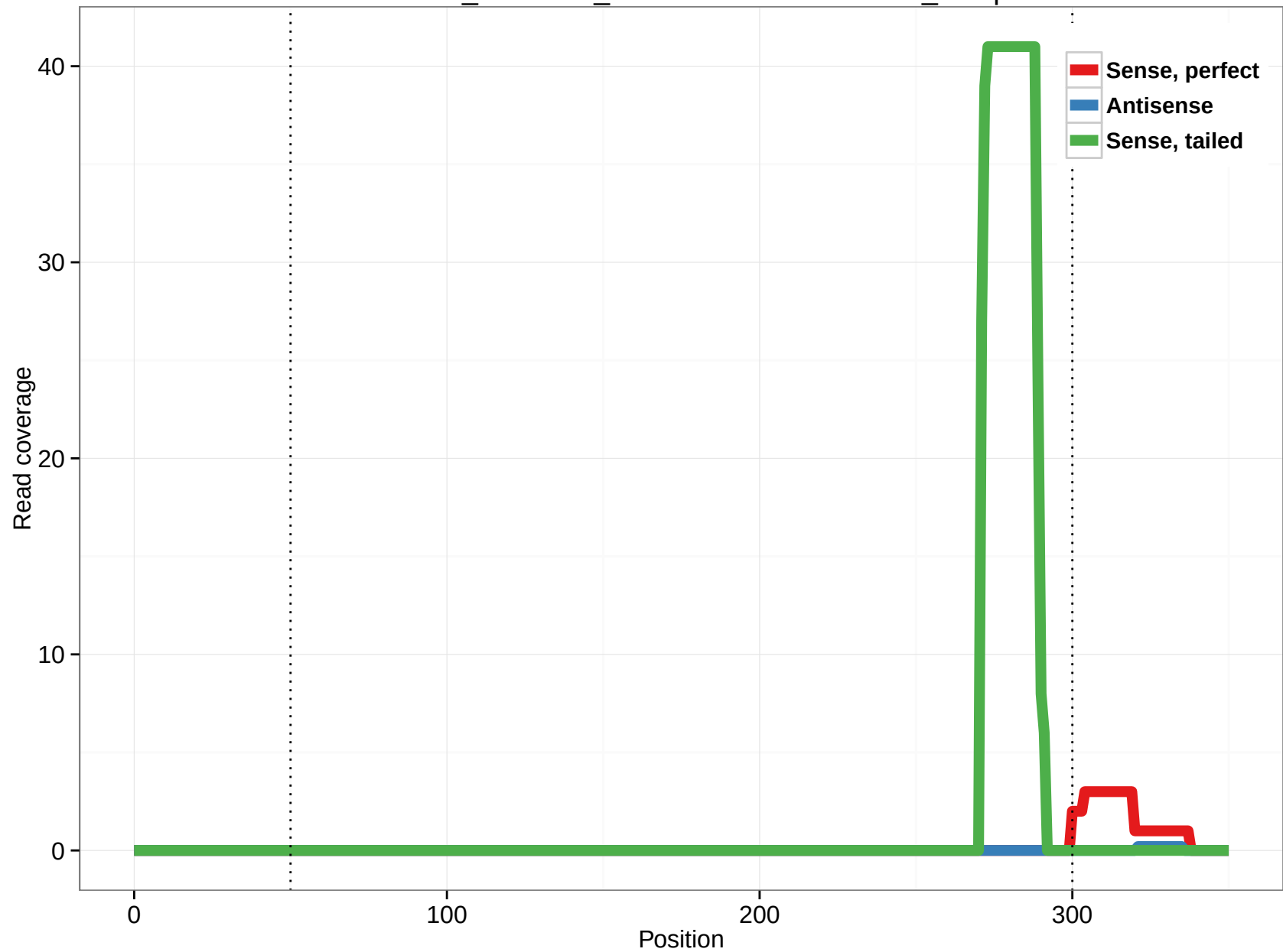
ornAna1_ensGene_ENSOANT00000017885_15.3p
