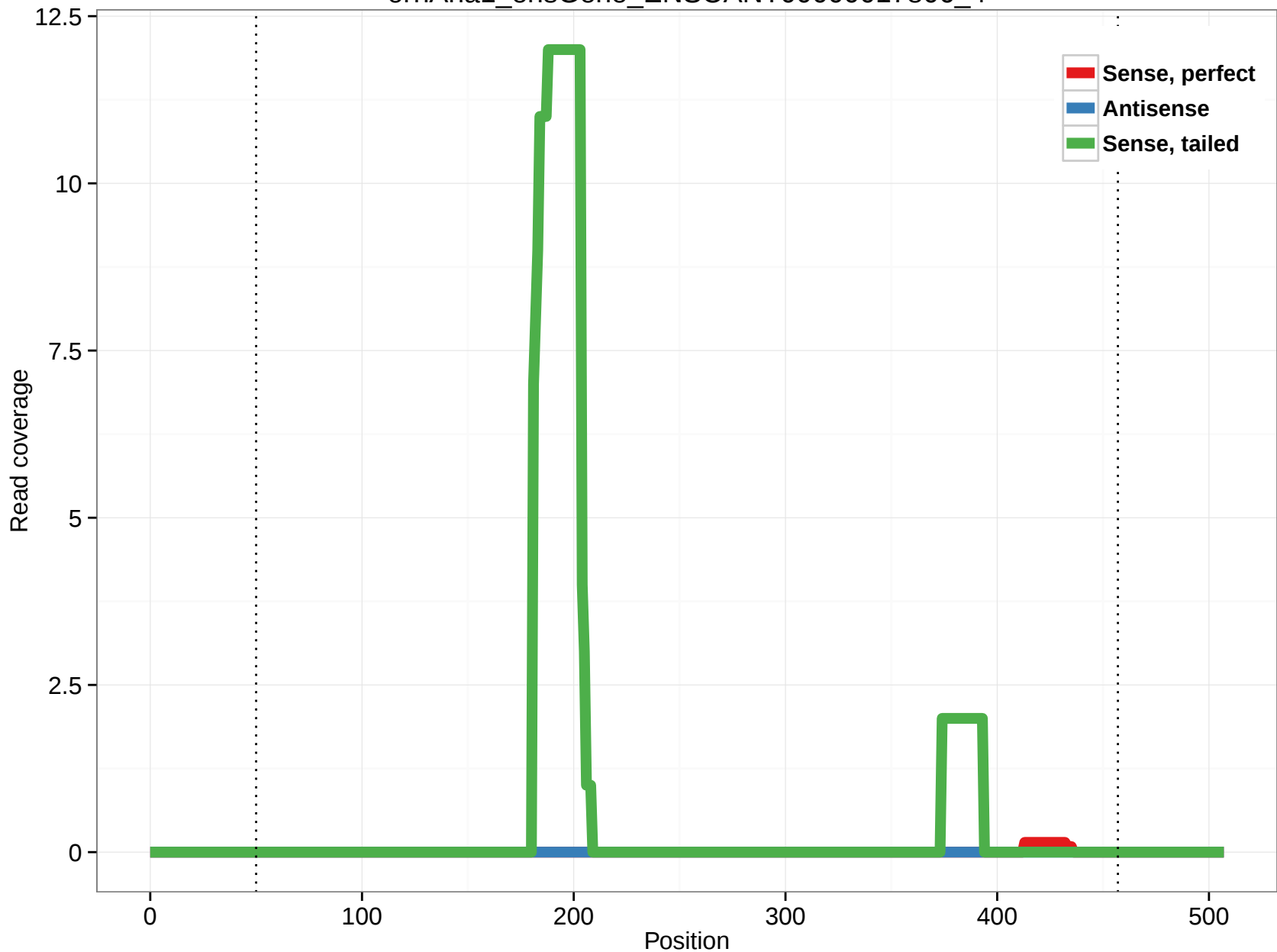
ornAna1_ensGene_ENSOANT00000017806_4
