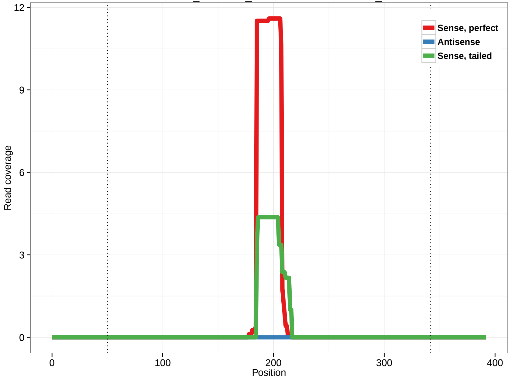
ornAna1_ensGene_ENSOANT00000017752_4
