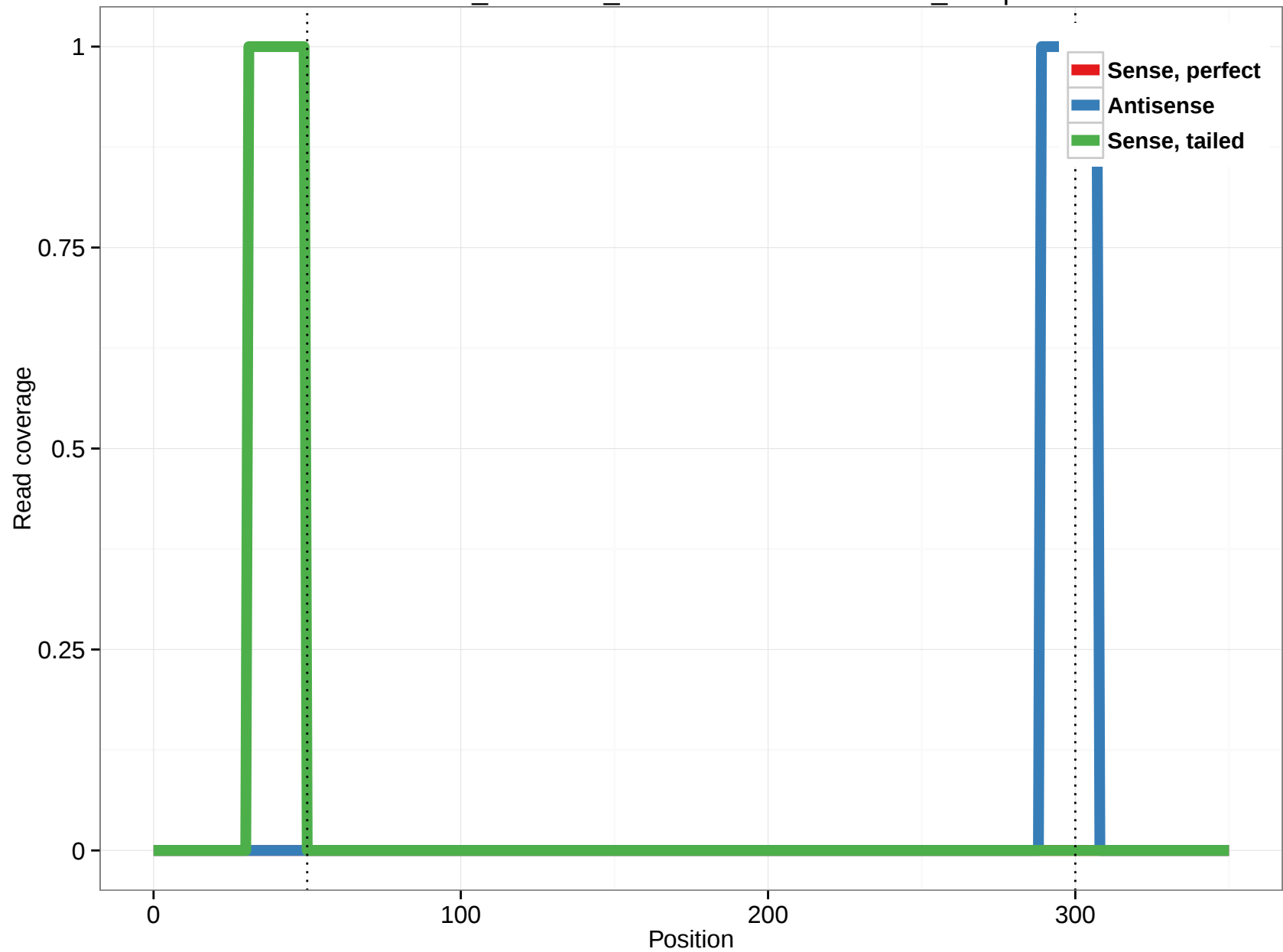
ornAna1_ensGene_ENSOANT00000017735_36.3p
