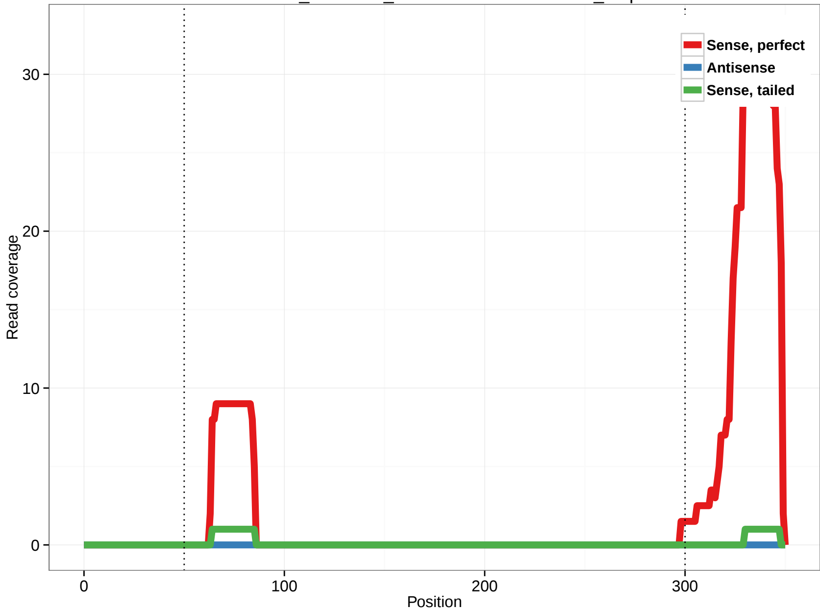
ornAna1_ensGene_ENSOANT00000017687_1.3p
