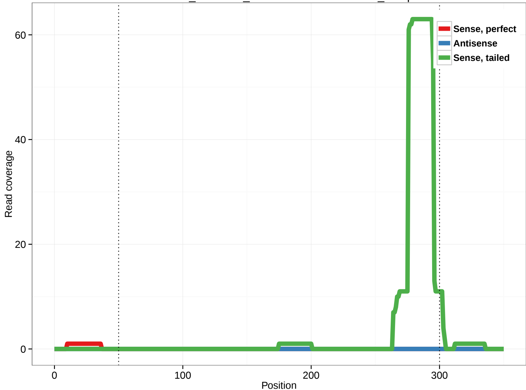
ornAna1_ensGene_ENSOANT00000017659_14.5p
