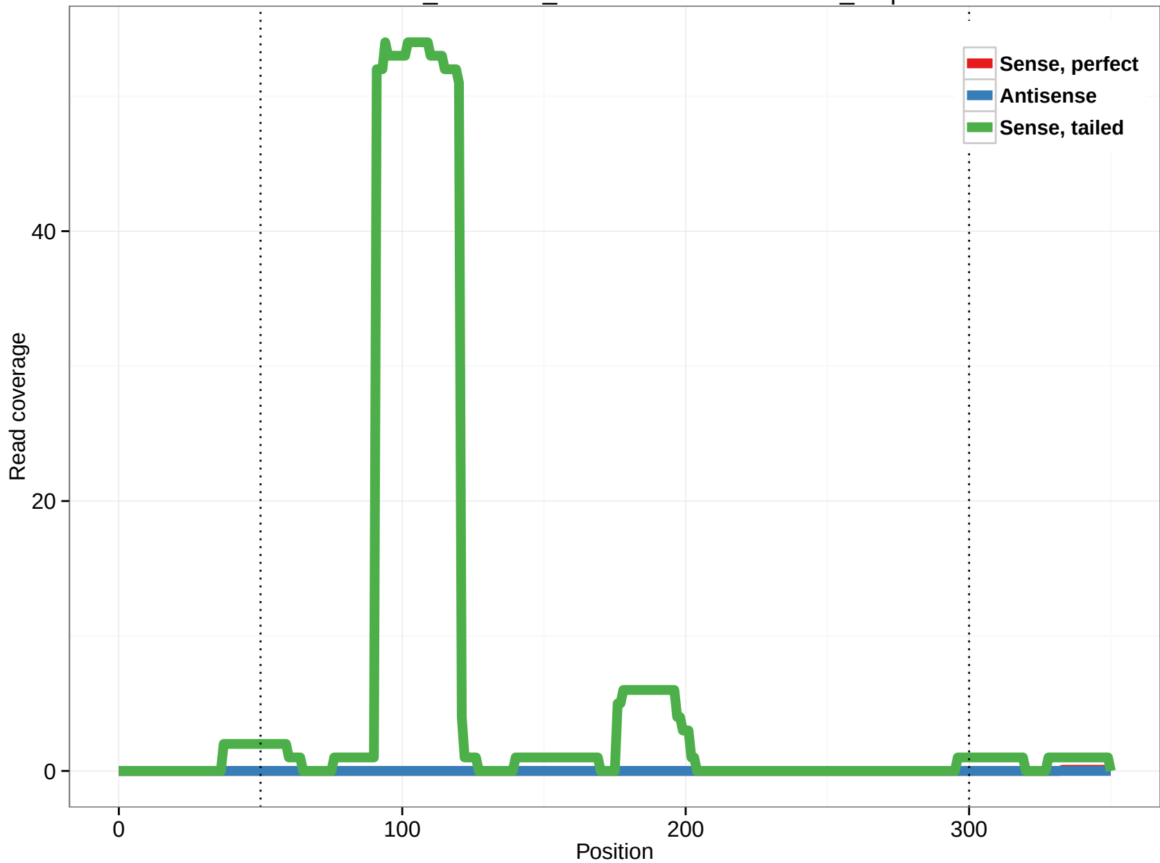
ornAna1_ensGene_ENSOANT00000017602_6.3p
