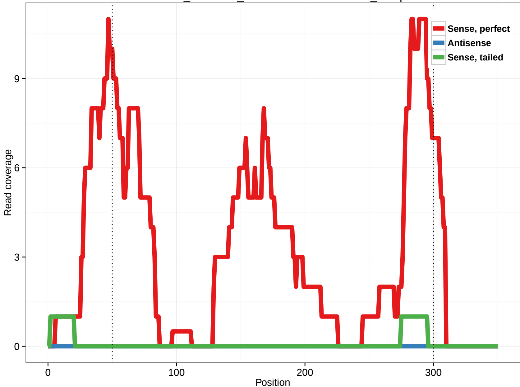
ornAna1_ensGene_ENSOANT00000017572_11.3p
