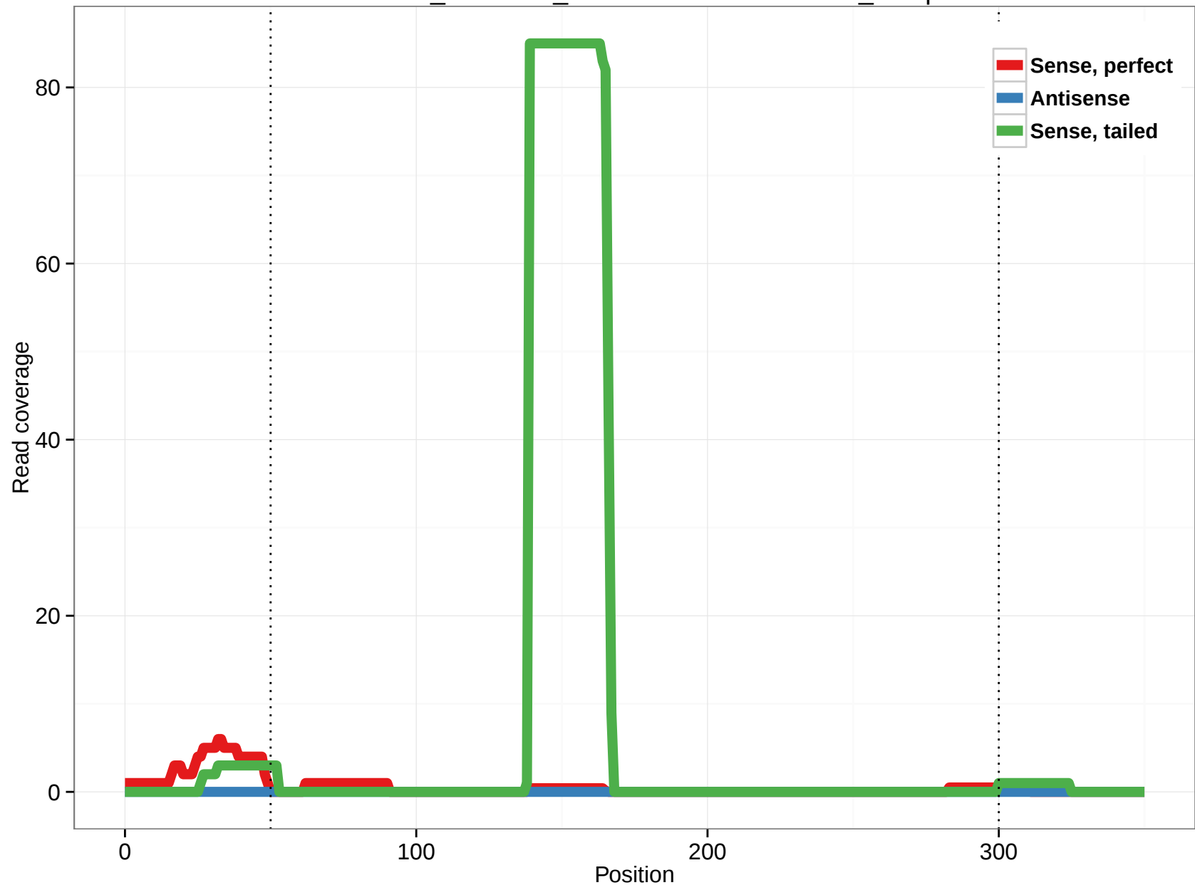
ornAna1_ensGene_ENSOANT00000017571_17.5p
