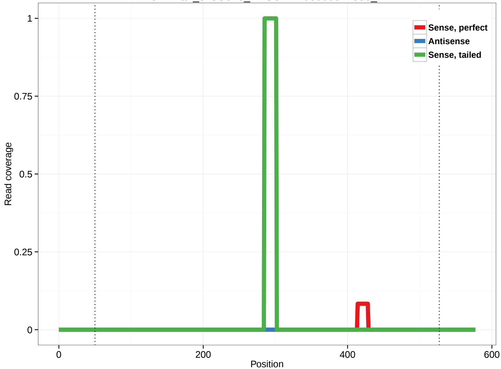
ornAna1_ensGene_ENSOANT00000017556_2
