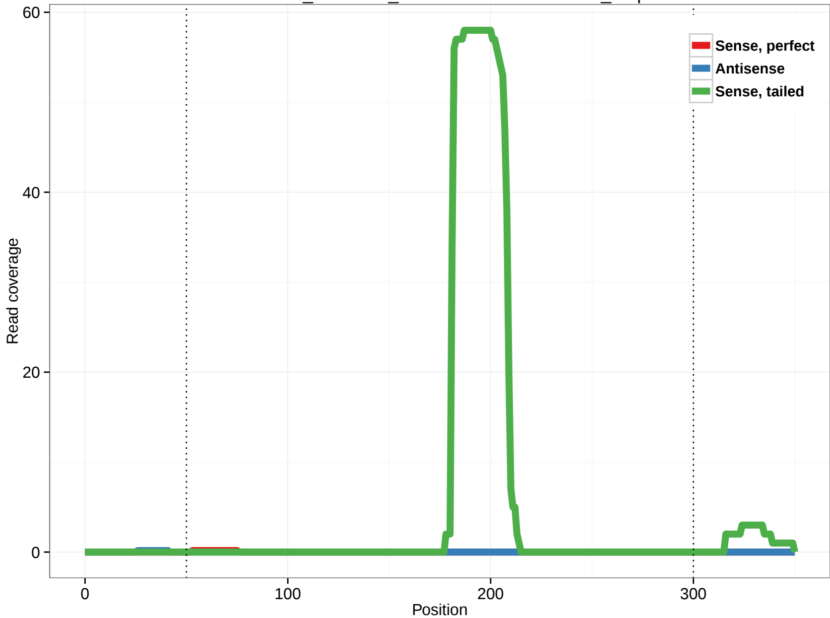
ornAna1_ensGene_ENSOANT00000017544_1.5p
