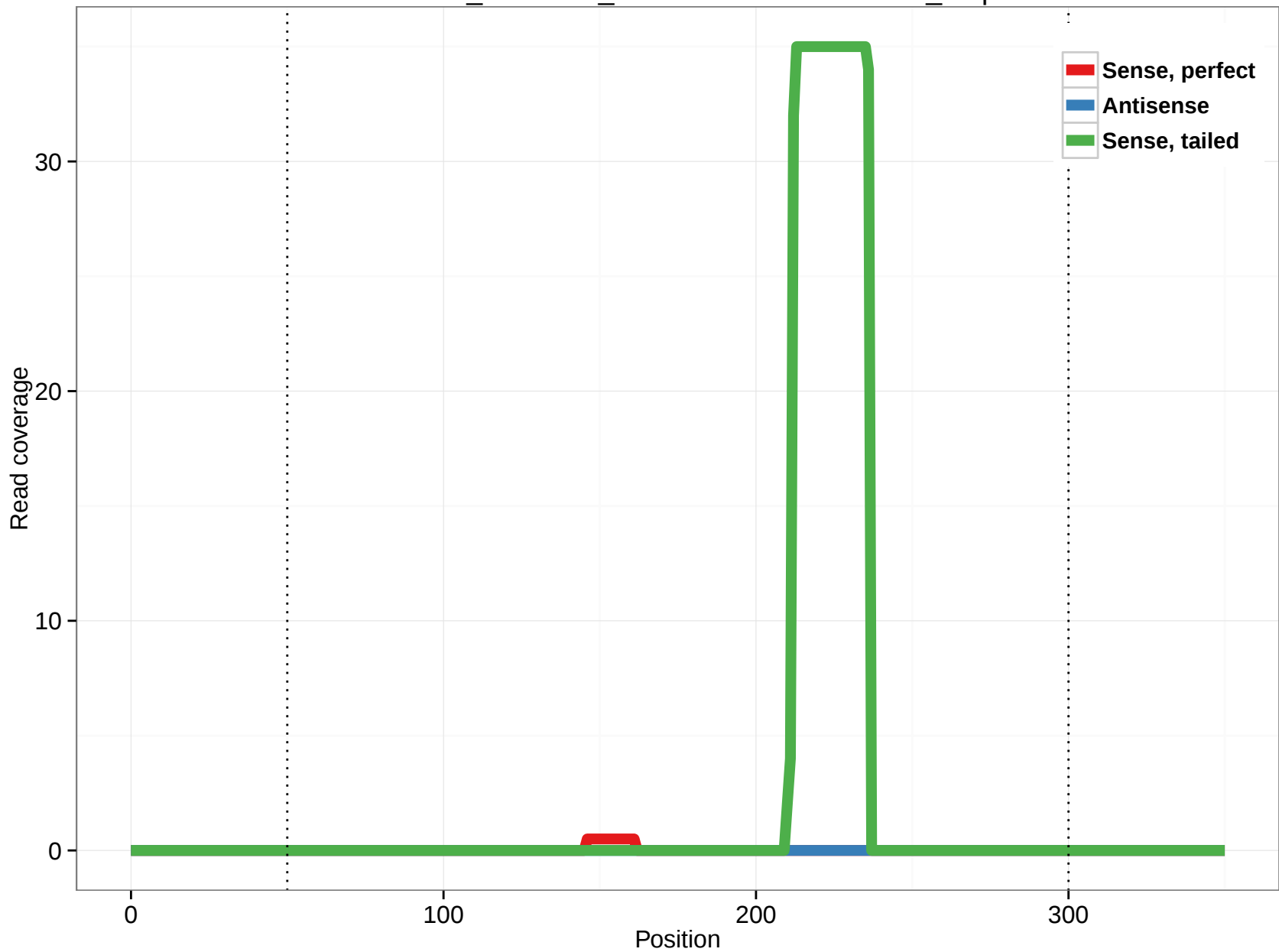
ornAna1_ensGene_ENSOANT00000017467_1.5p
